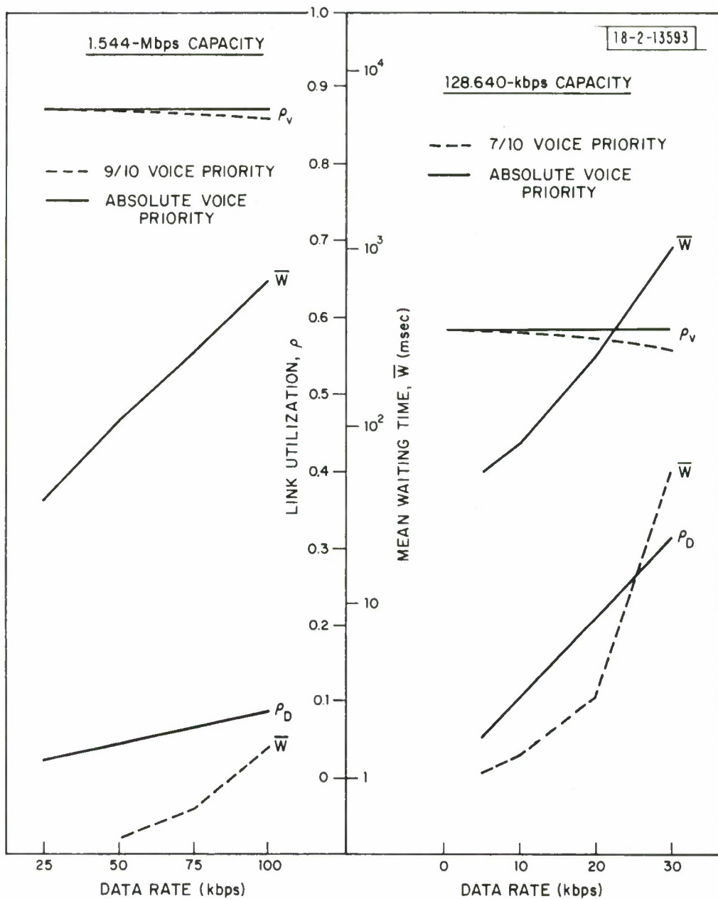
Fig. 7. Link utilizations for voice and data (linear scale). Mean waiting times for data packets (logarithmic scale). Solid curves: absolute voice priority. Dashed curves: indicated voice/data priority (see text).
