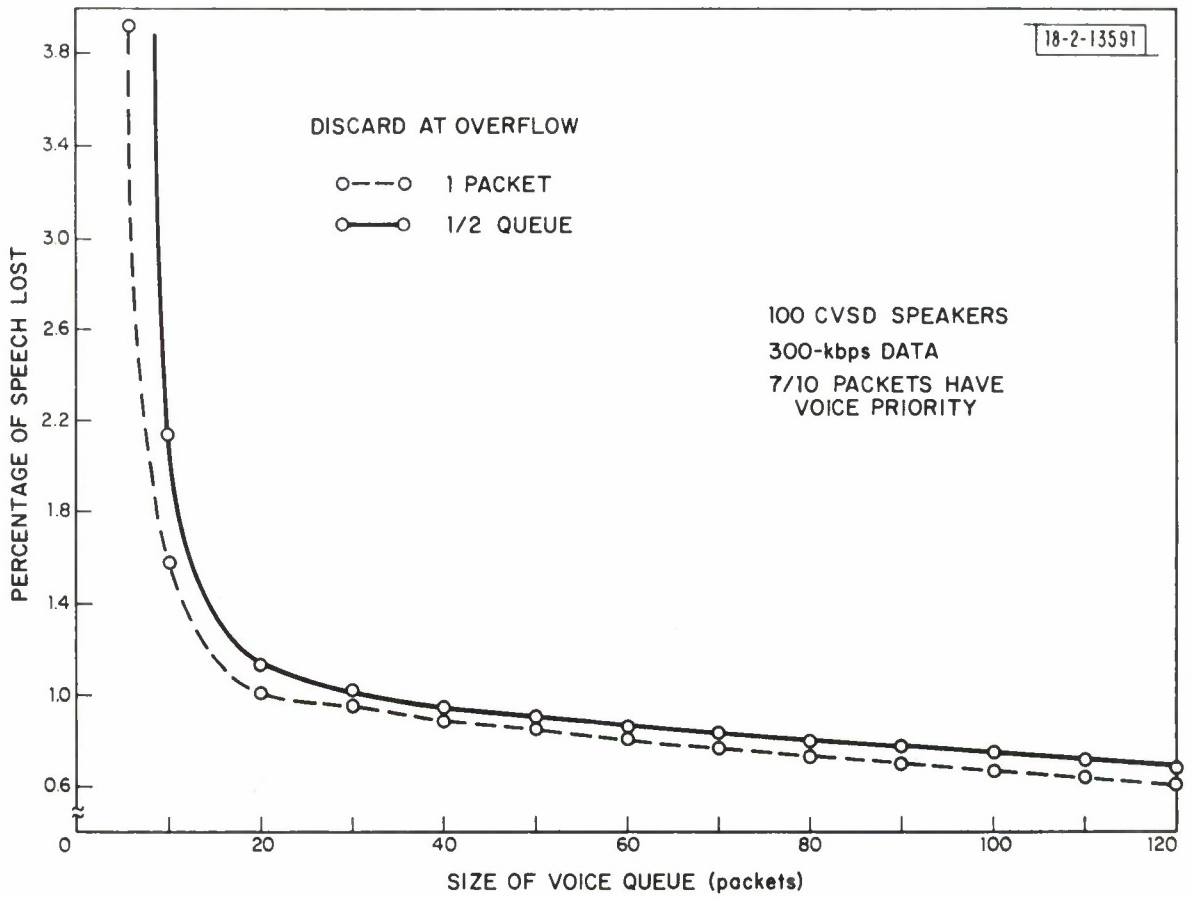
Fig. 5. Speech loss vs. size of voice queue.
