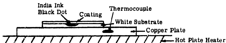
Figure 1. Emissivity Test.
