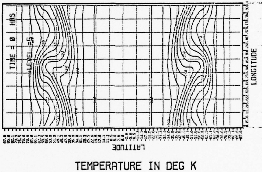
Figure 8. Initial high resolution temperature for \sigma = .9 . Contour interval is 5°K.
