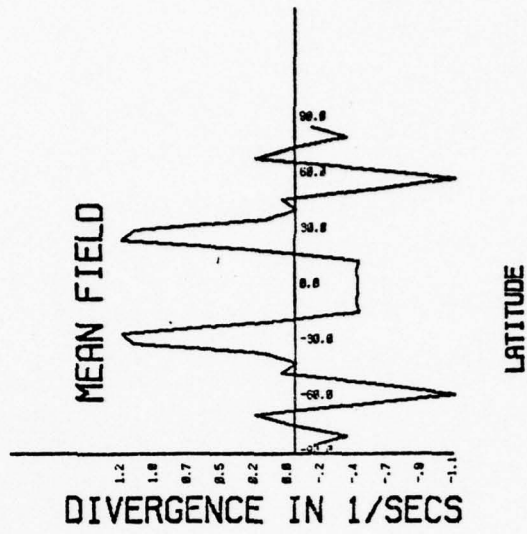
Figure 6. Initial low resolution divergence for \sigma = .9 . Contour interval is 1 \times 10^{-6} \text{sec}^{-1} . Mean field is scaled by 106.
