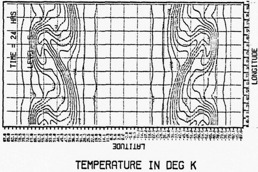
Figure 12. 24 hr high resolution temperature for \sigma = .9 . Contour interval is 5°K.
