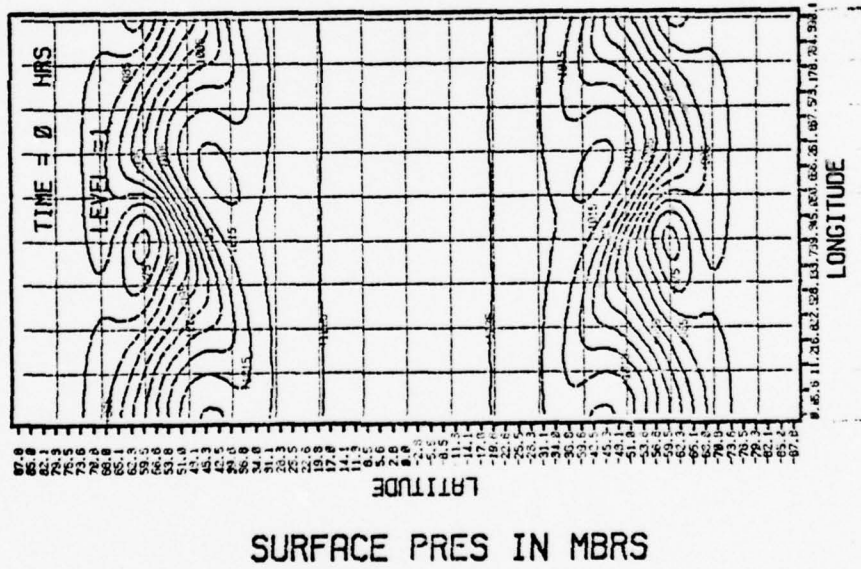
Figure 7. Initial high resolution surface pressure. Contour interval is 5 mb.
