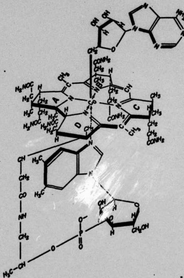
SPATIAL STRUCTURE OF COENZYME B 12
