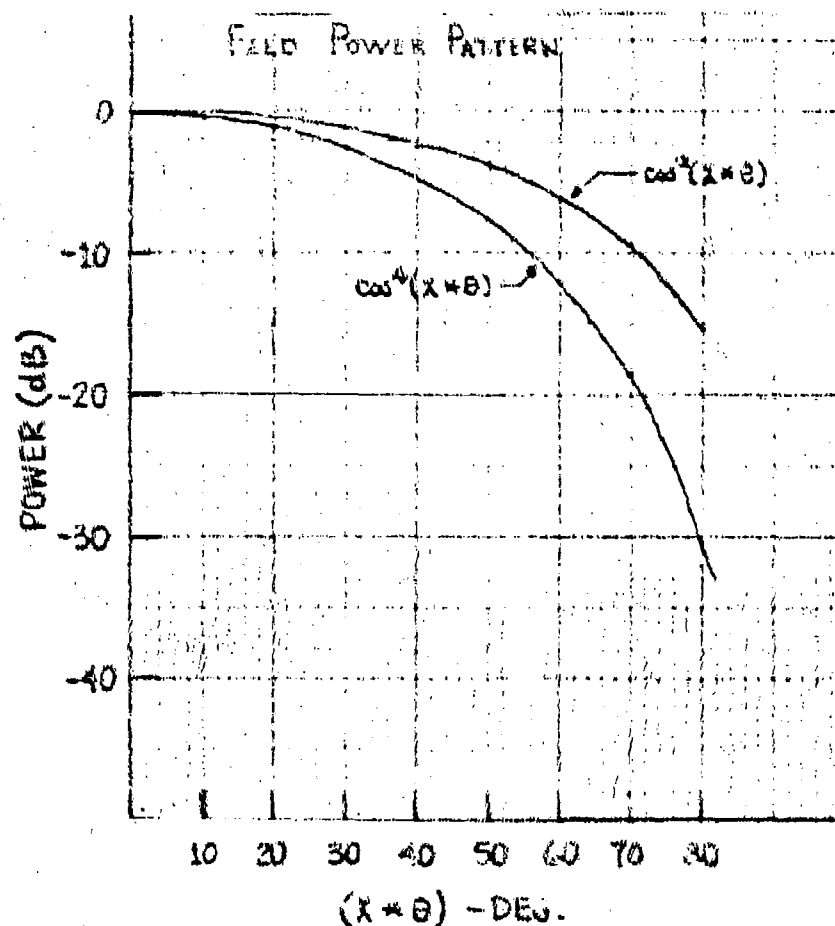
Figure 5-15. Feed Power Patterns [ -2(\theta) = \cos^2(x\theta) ]
