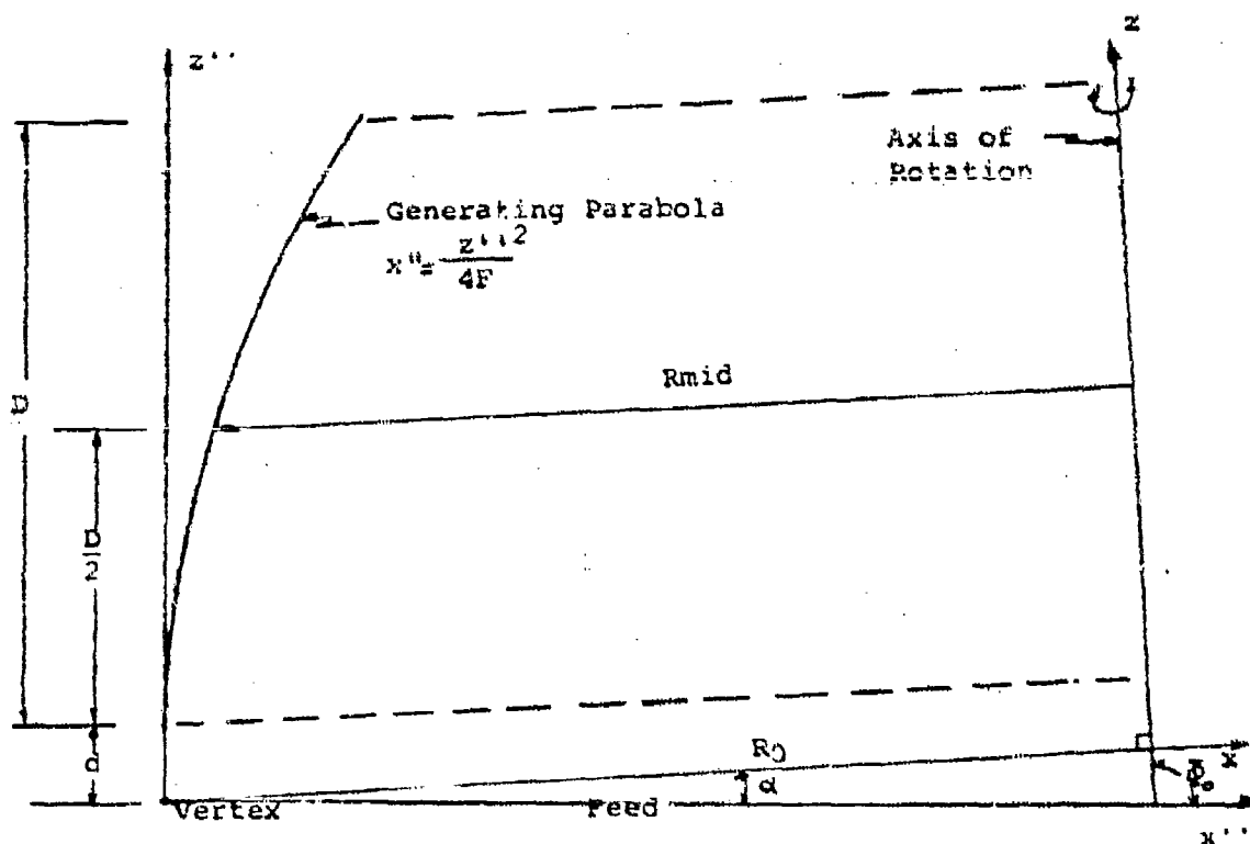
Figure 6-9. Reflector Geometry
