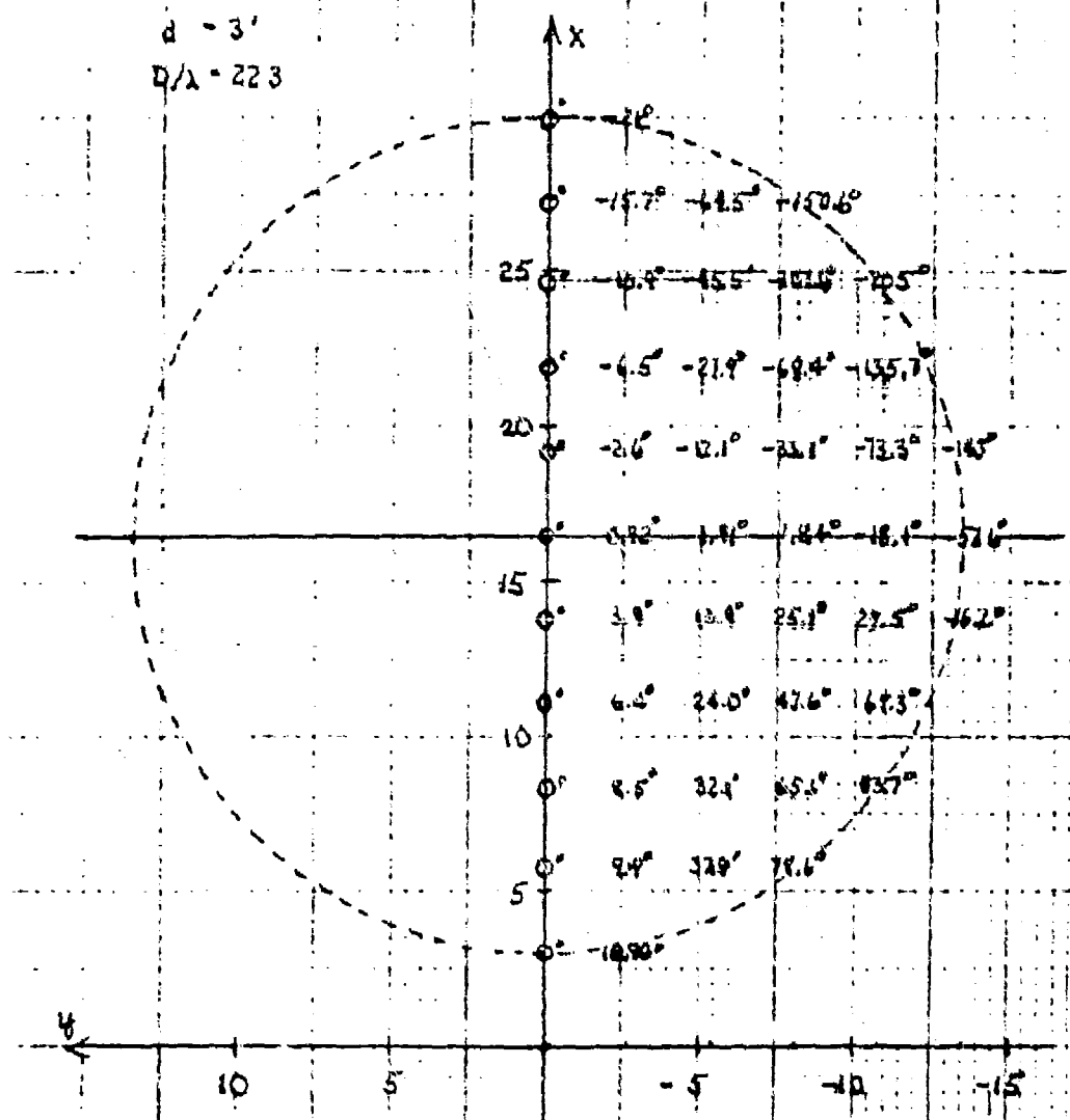
Figure 5-29. Offset (11%) MBTA ( D/R = 0.4 ) Aperture Plane Phase Errors with Optimum Focusing
