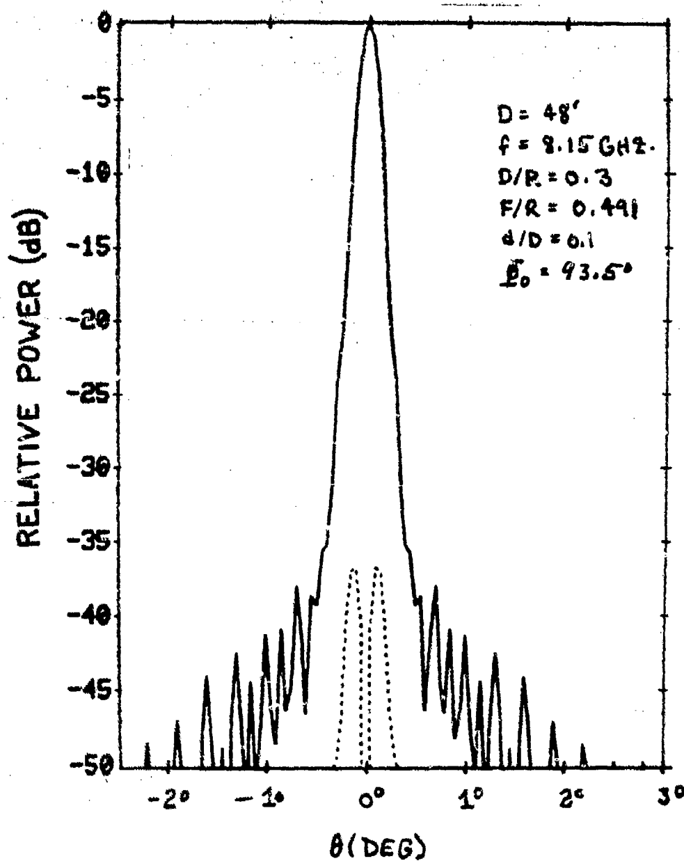
Figure 5-58. 48-ft-Diameter MBTA ( D/R = 0.3 ) Pattern at 8.15 GHz ( \bar{\theta} = 90.2^\circ )
