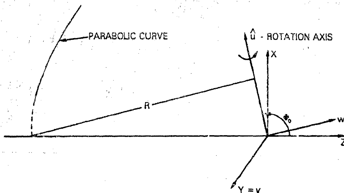
Figure 5-20. Geometry for MBTA Reflector Equation
