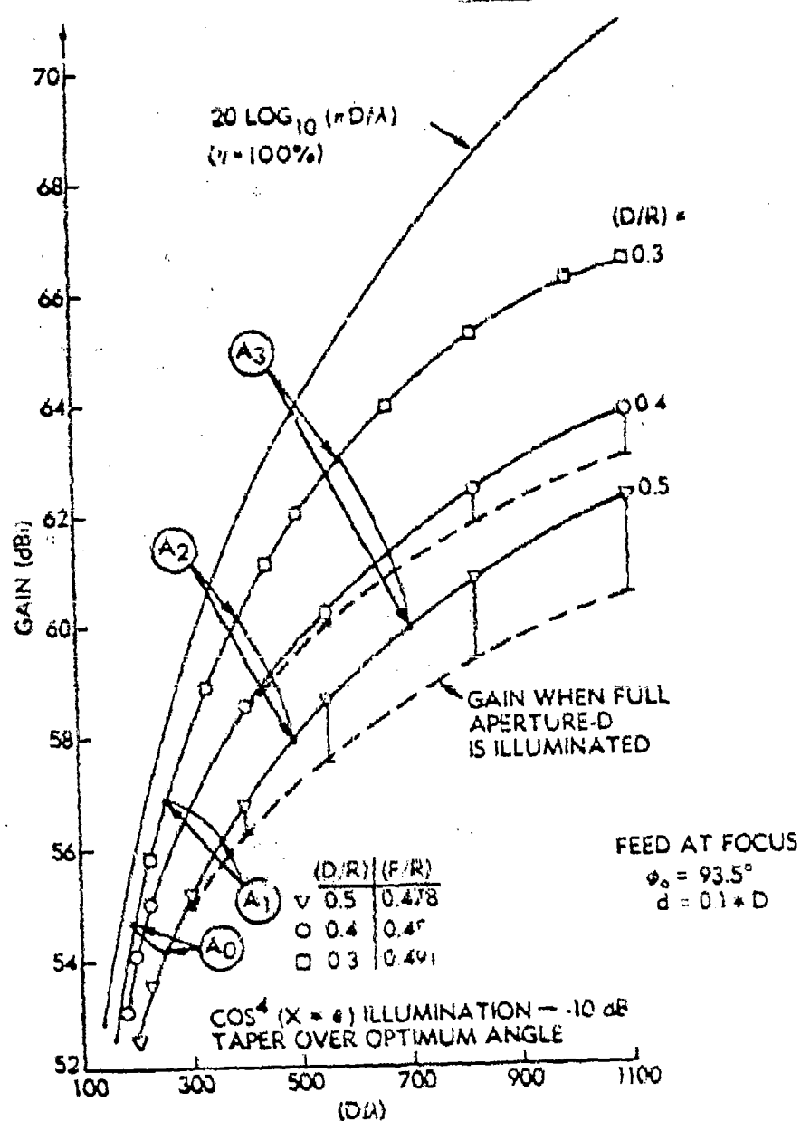
Figure 5-44. Illumination Gain with Equal Projected Area Contours
