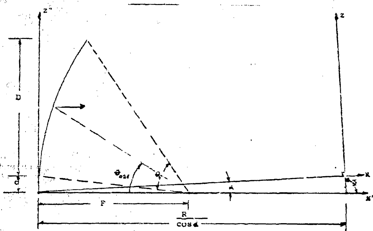
Figure 6-1. Offset Feed Configuration
