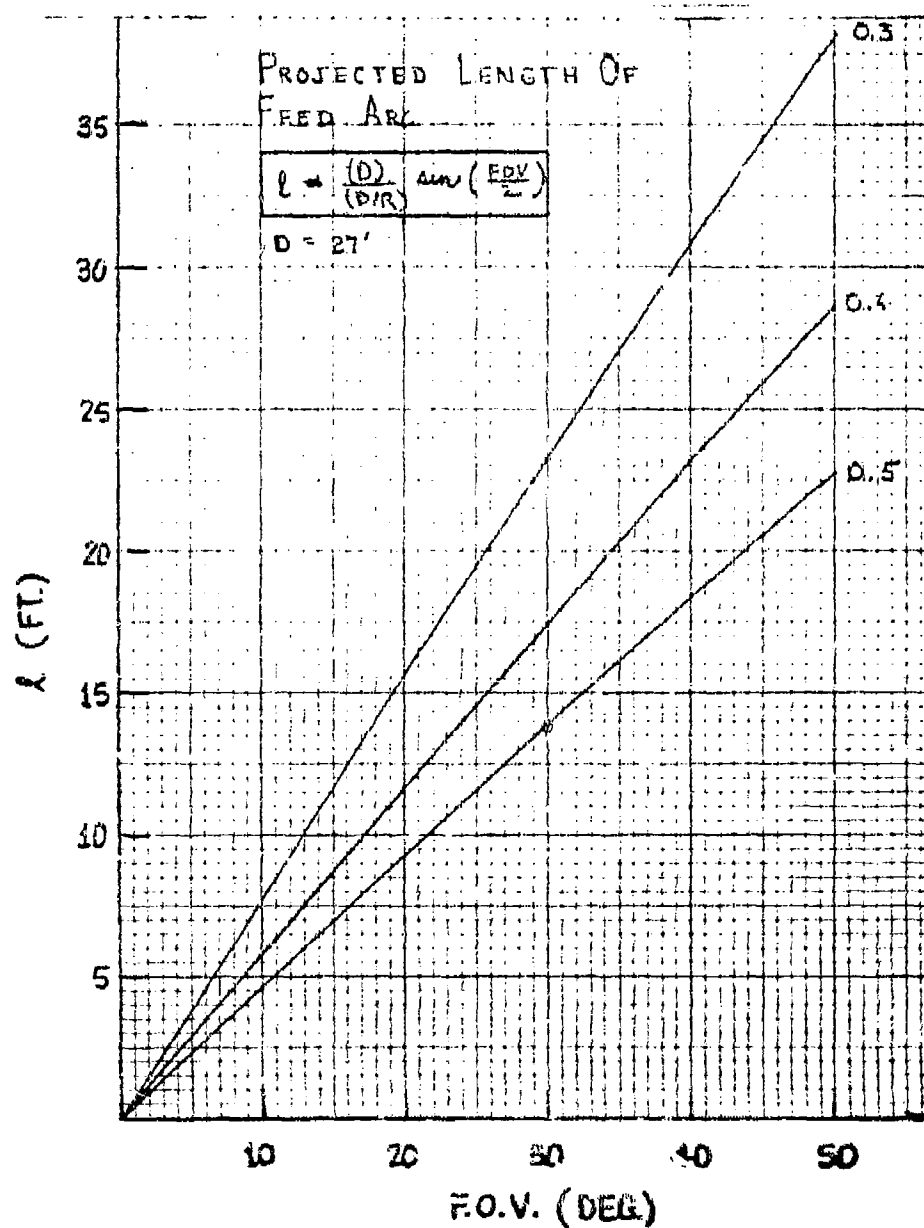
Figure S-8. Projected Length of Feed Arc for 27-ft-Diameter Symmetrical MBTA
