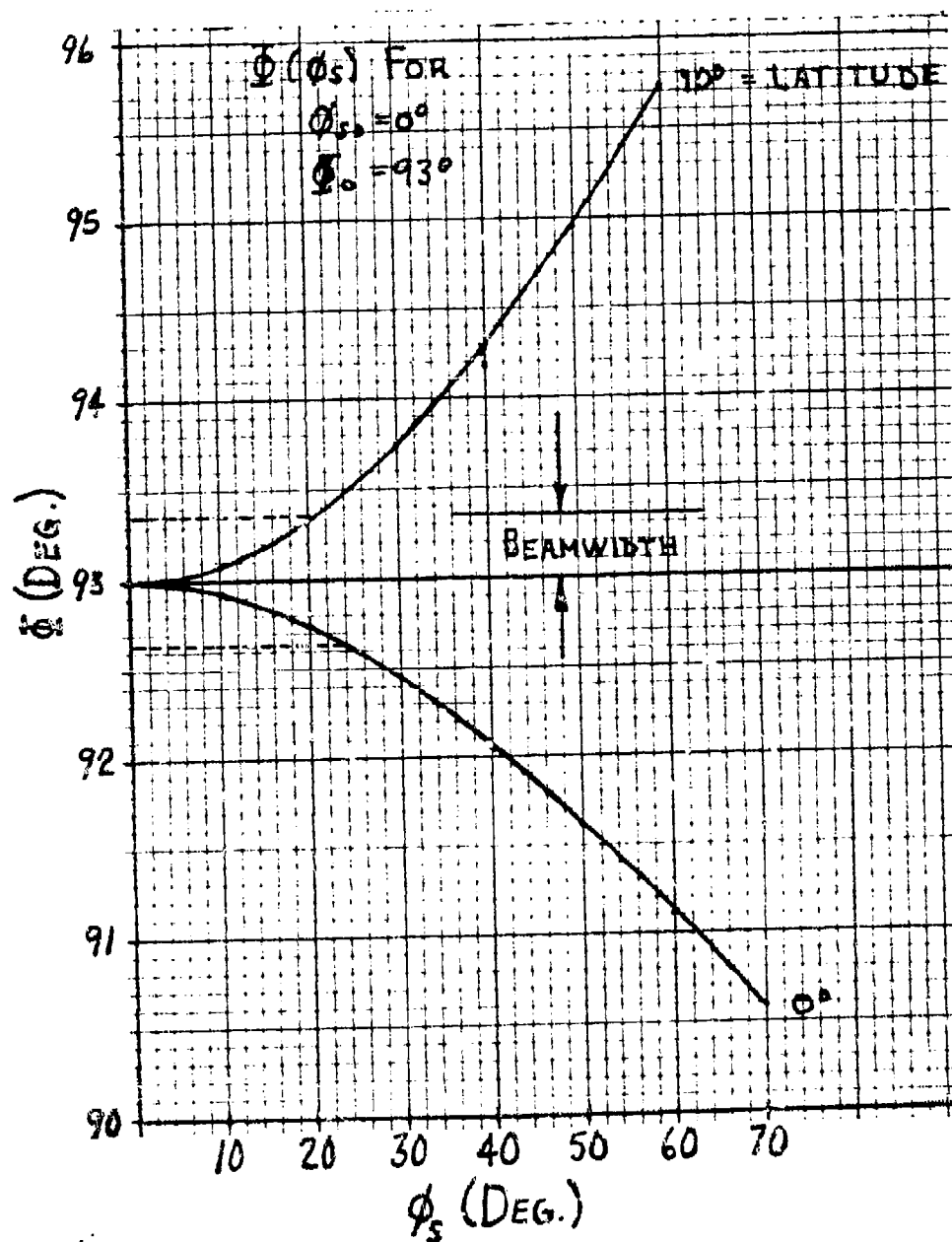
Figure 4-18. \phi(\phi_s) for \phi_0 = 93^\circ , \lambda = 0^\circ
