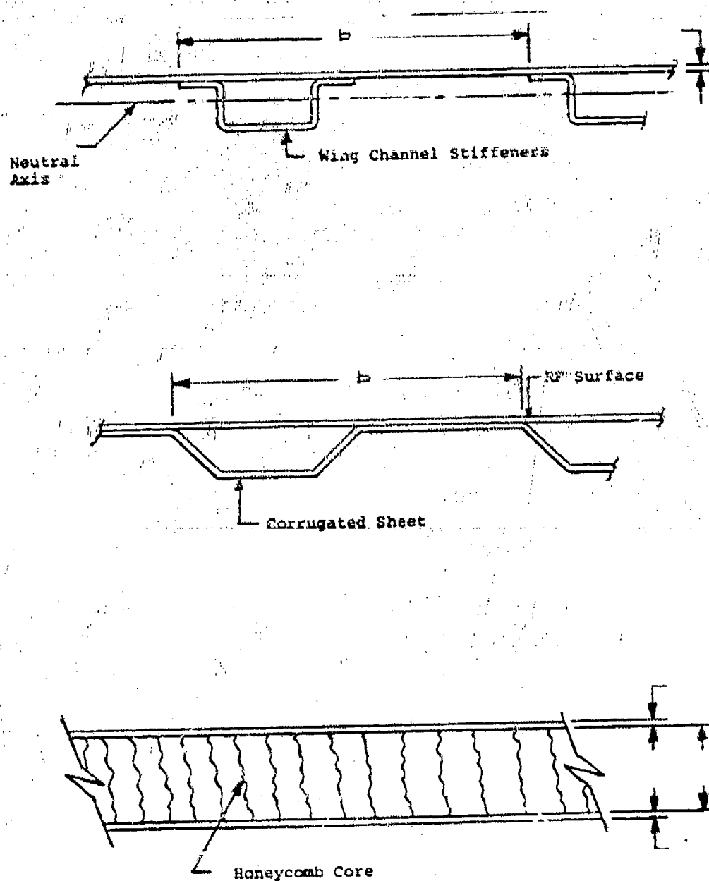
Figure 6-16. Reflector Panel Cross Section
