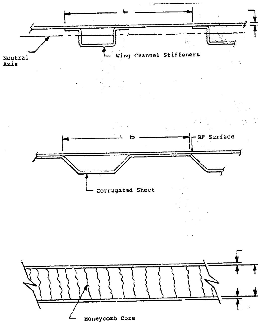
Figure 6-16. Reflector Panel Cross Section
