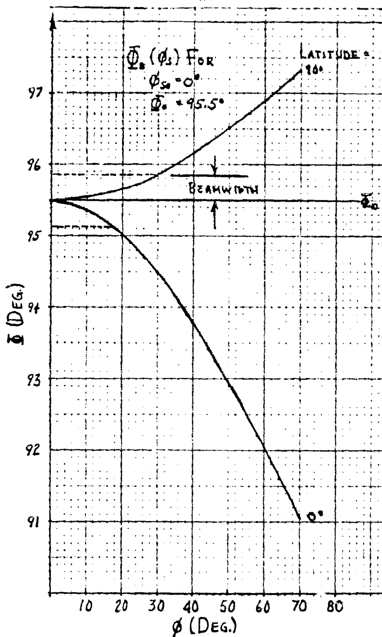
Figure 4-21. \bar{\phi}(\phi_s) for \phi_0 = 95.5^\circ , \lambda = 0^\circ
