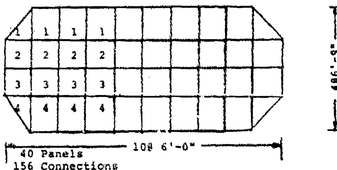
Figure 6-17. Panel Configurations
