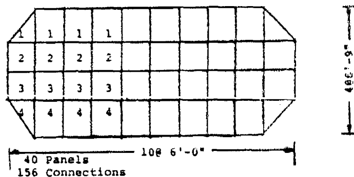
Figure 6-17. Panel Configurations
