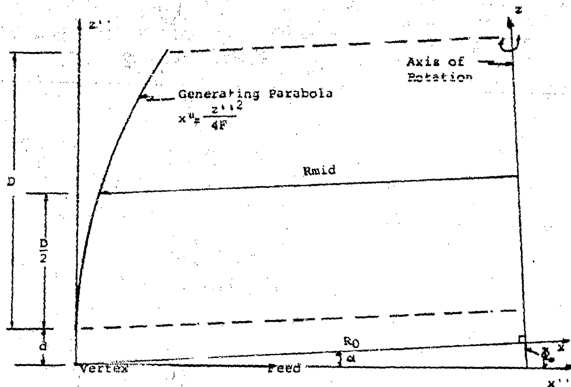
Figure 6-9. Reflector Geometry
