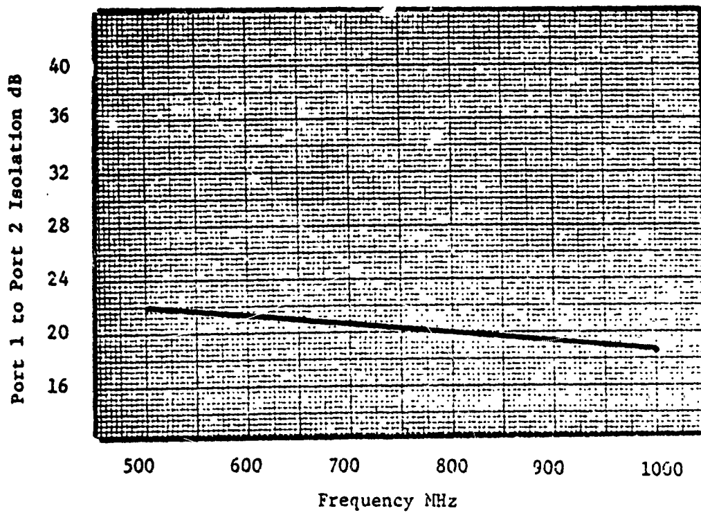
Figure 36. Isolation Plated Up Coupler #2.
