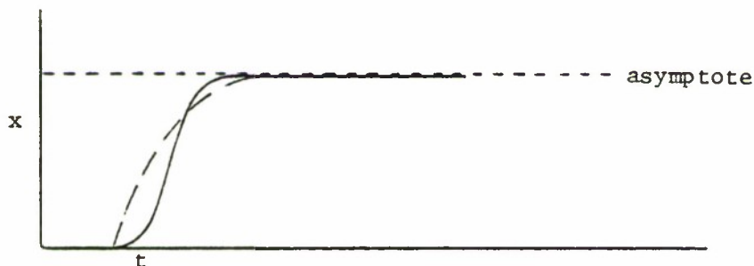
Fig. 5.1—Logistic Curve
