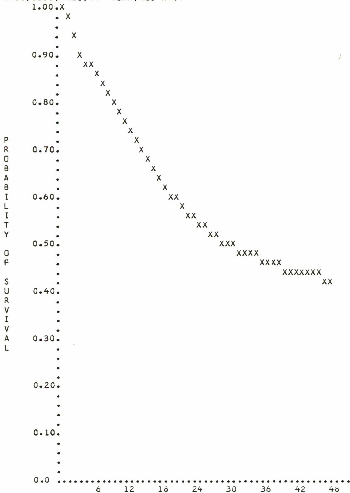
Fig. 7.4—Survival Function
