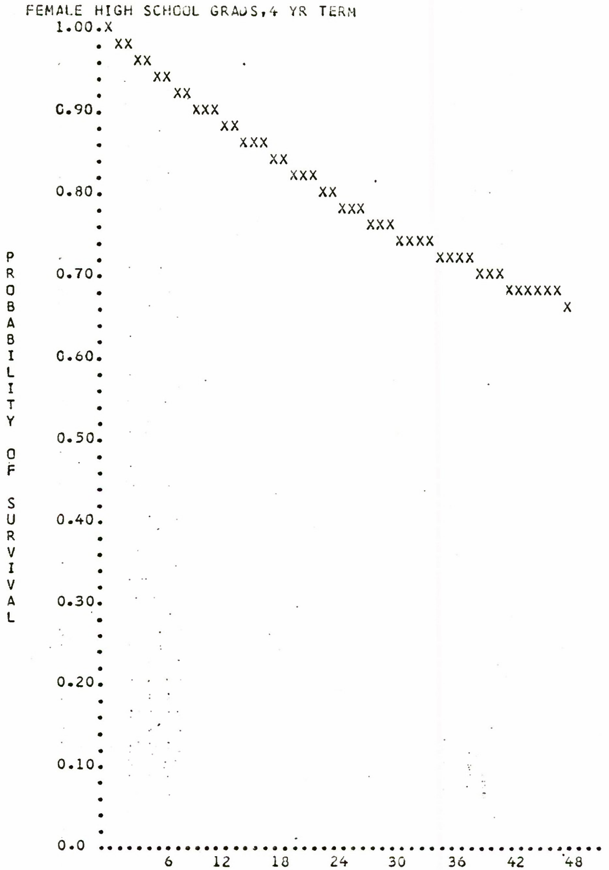
Fig. 7.7—Survival Function
