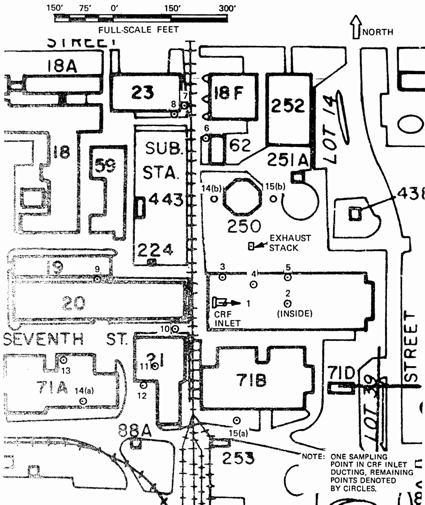
Figure 8 NEAR-FIELD SAMPLING POINT LOCATIONS FOR DETERMINING TEMPERATURE RISE ABOVE AMBIENT
