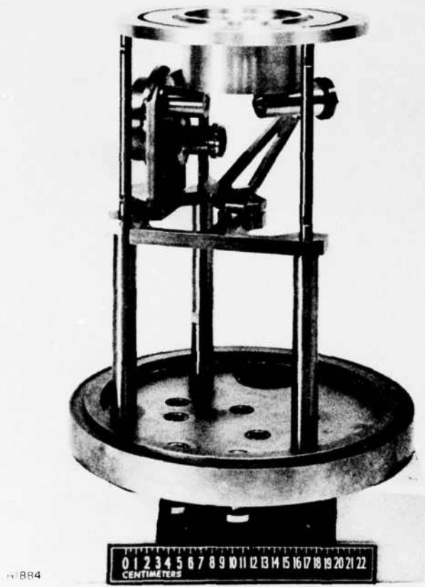
4884 Figure 3 Photograph of the E-Gun and Hemispherical Electrostatic Analyzer
