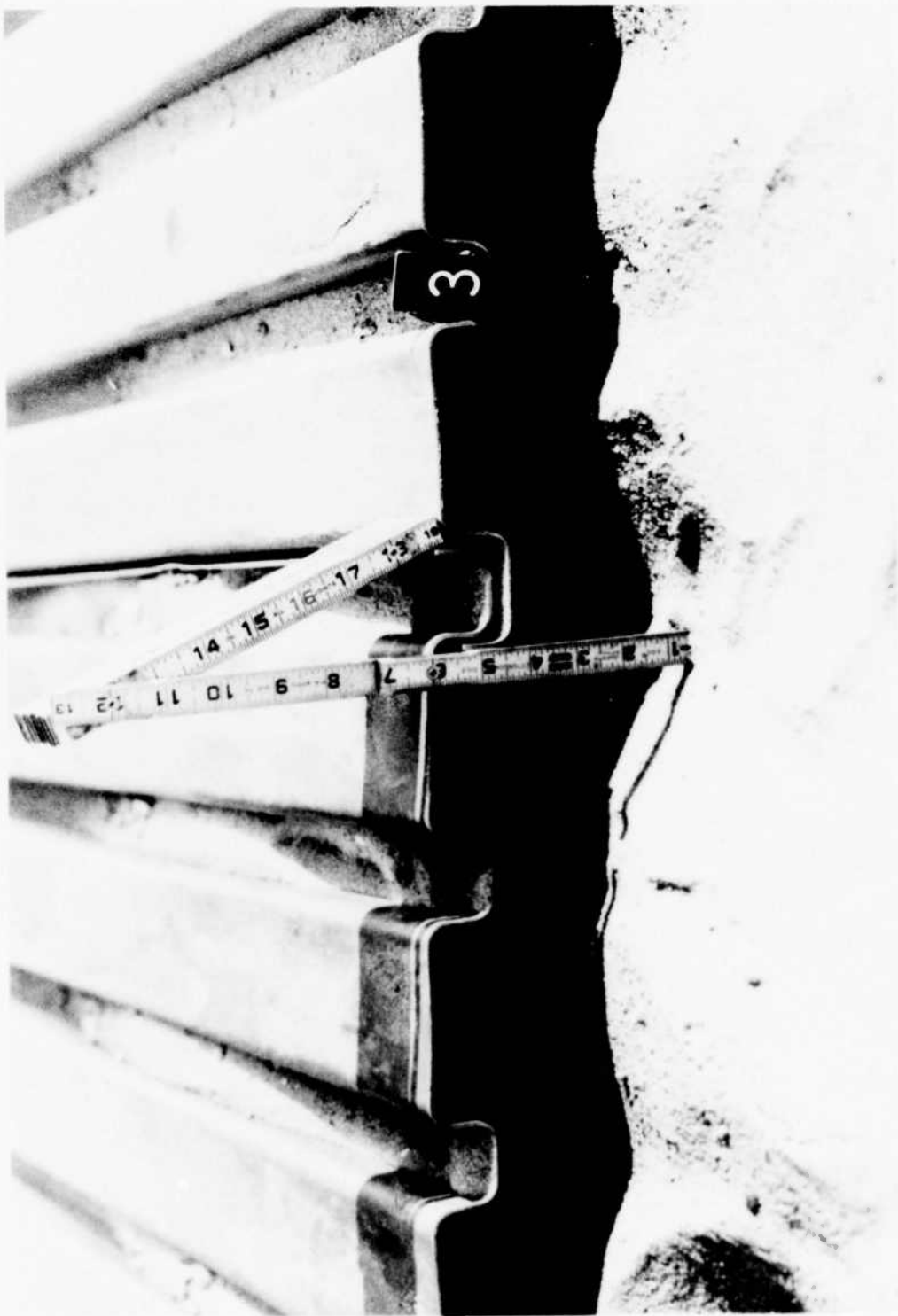
Photo 14. South edge of Fletcher panels after 1000 passes
