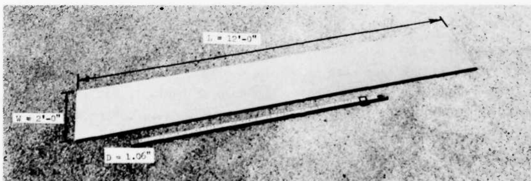
Figure 18. Spur-Ecolite aluminum, 1- by 1-in. core and two-skin sandwich panel
