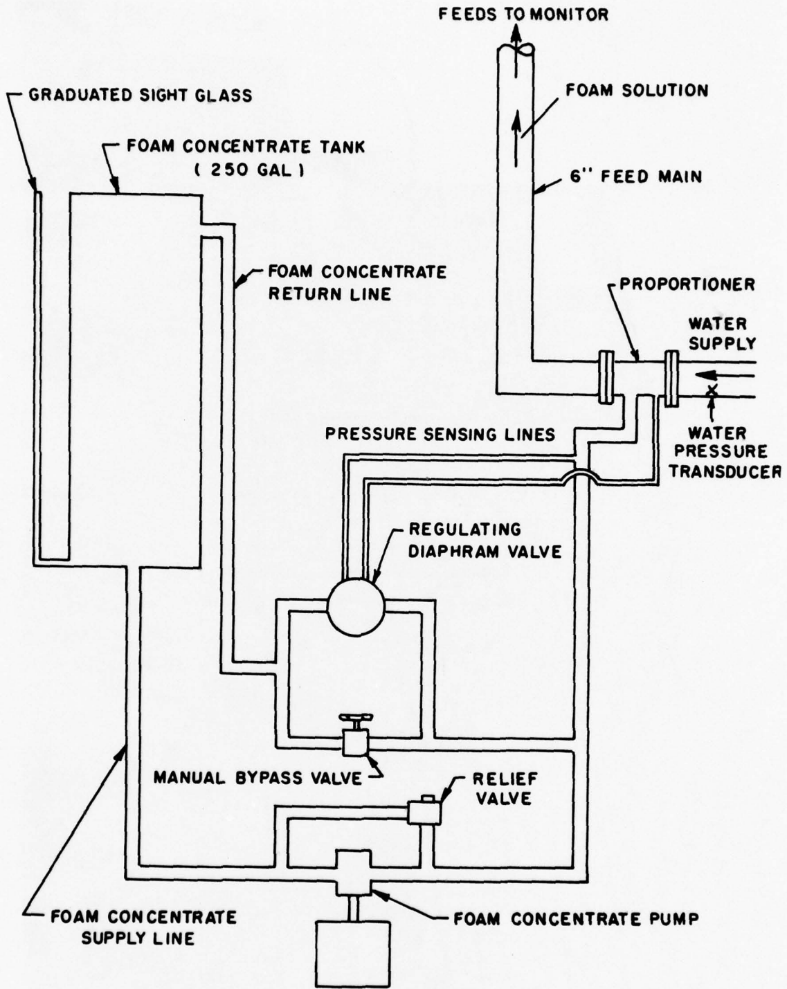
FIGURE 5 PROPORTIONING SYSTEM
