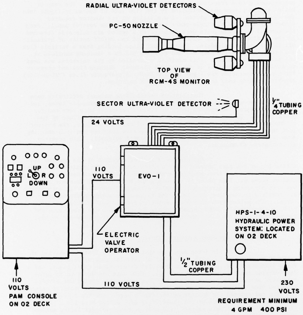
FIGURE 22 PROGRAMMED AUTOMATIC MONITOR
