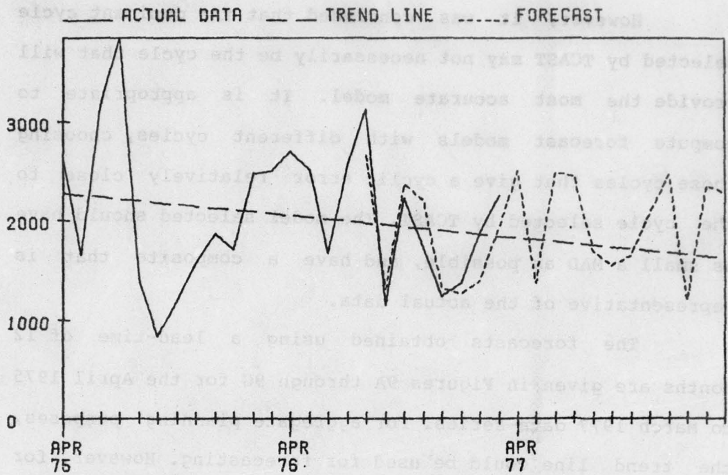
Figure 9A. GRAPH: BAJOBS, FORECAST AND TREND
