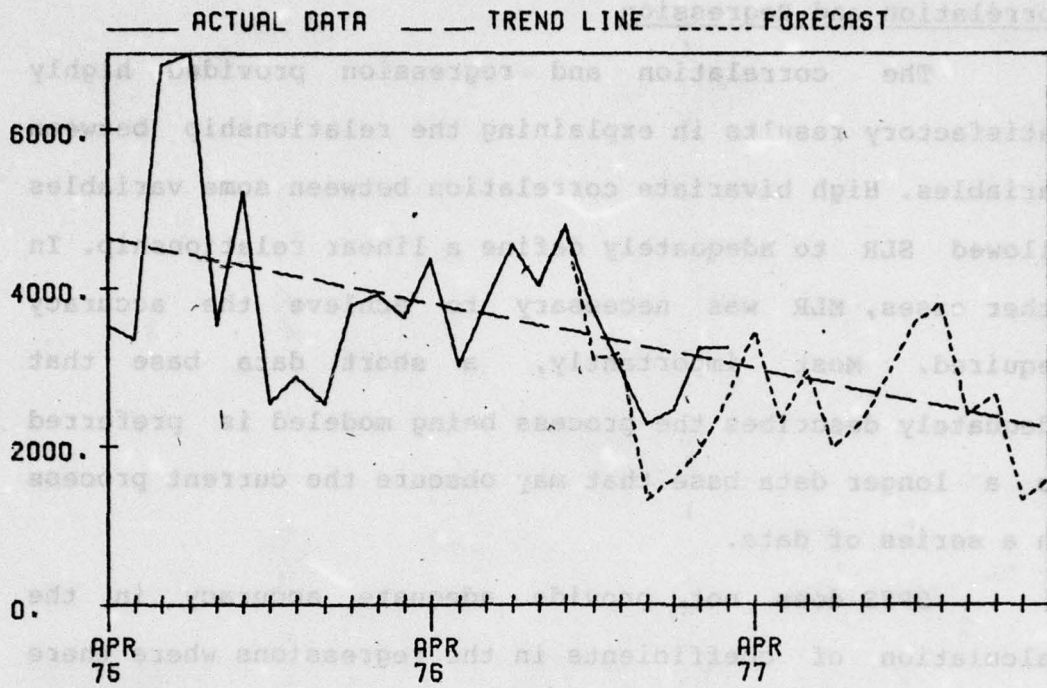
Figure 9G. GRAPH: LOGONS, FORECAST AND TREND
