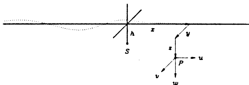
Figure 1. Cartesian Coordinates. Position of a point P with respect to the source S .
