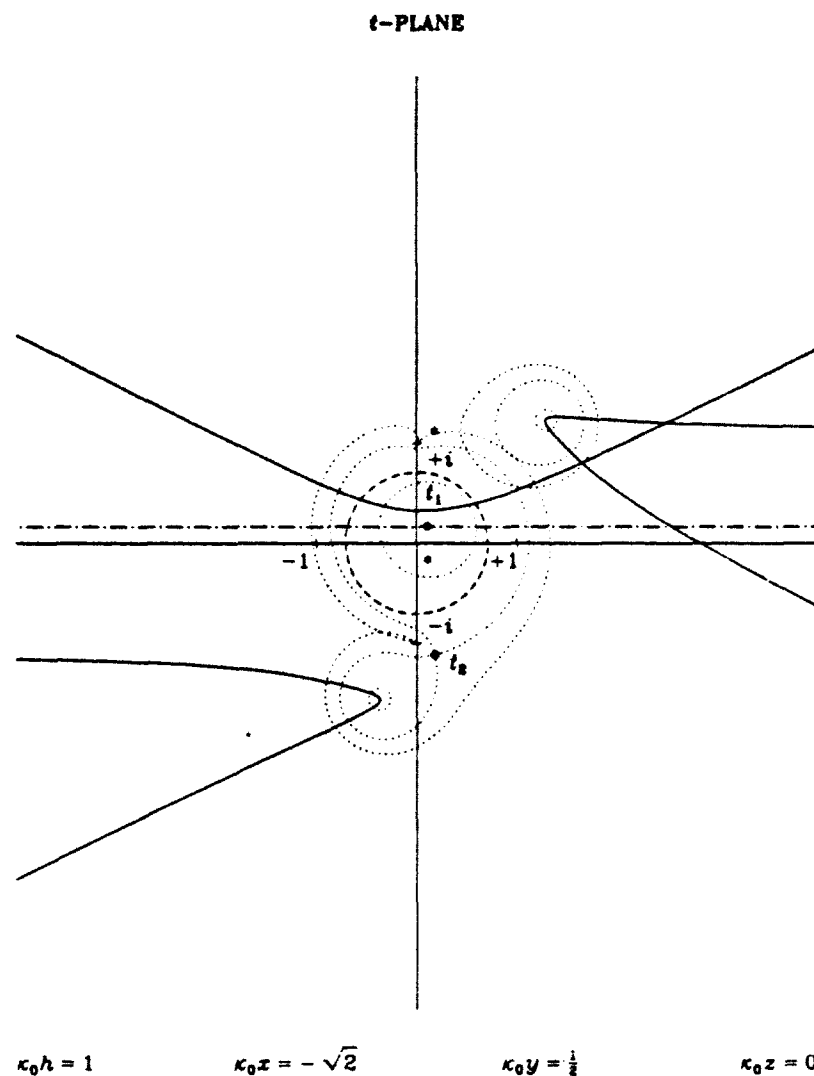
Figure 4. Azimuthal Integration with respect to Wave Number. •, primary singularities; •, secondary singularities; ---, circle of radius \frac{1}{\sqrt{2}} ; ---, boundary of convergence; —, primary branch, natural path; —, secondary branch, natural path; ---, actual path of integration.
