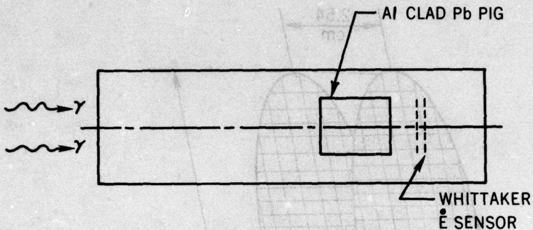
Figure 22. Floating pig.
