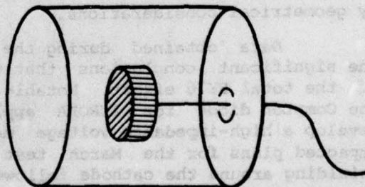
Figure 2. Compton diode.
