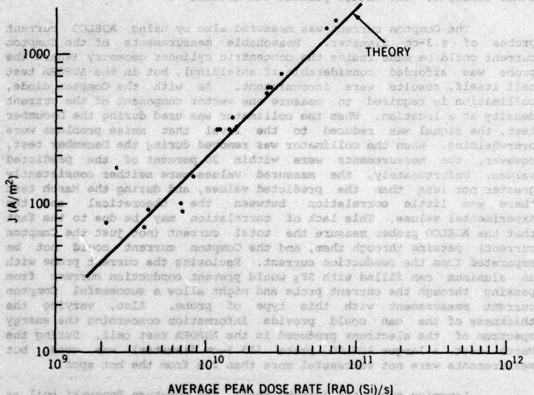
Figure 16. \dot{J} sensor.
