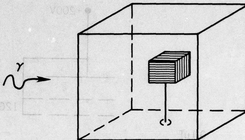
Figure 4. Concentric box test geometry.
