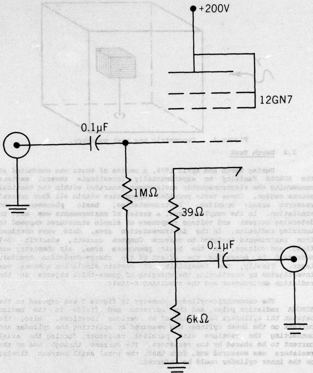
Figure 3. Cathode follower.
