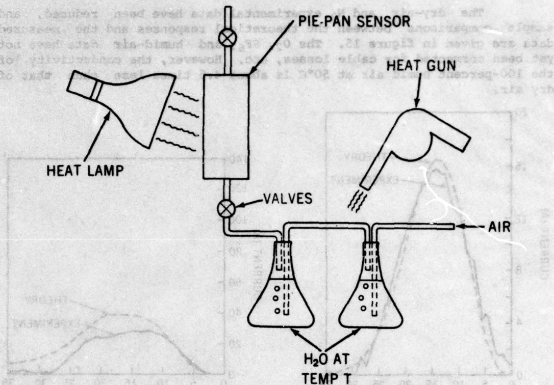
Figure 13. Method of filling pie-pan sensor with humid air.
