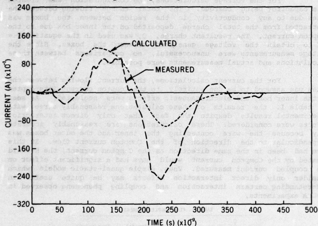
Figure 19. Total axial current on inner cylinder.
