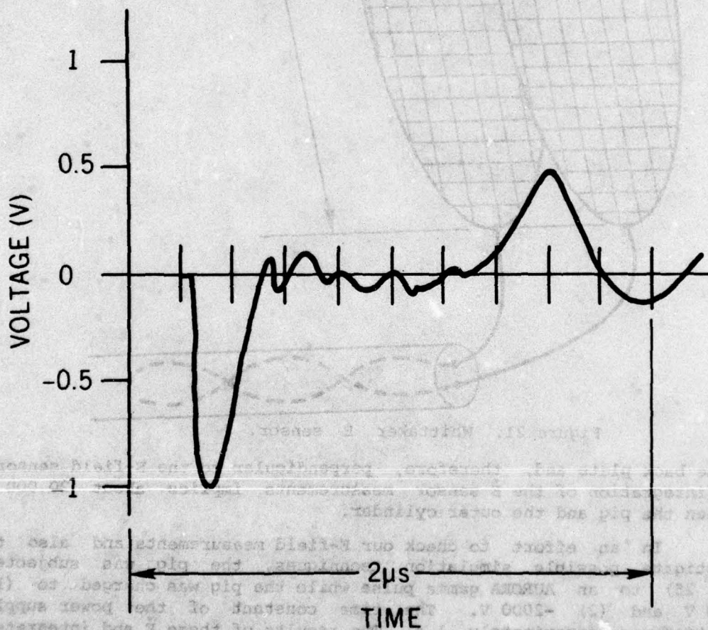
Figure 23. Output of E sensor (oscilloscope trace).
