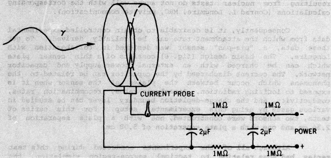
Figure 8. Pie-pan sensor.
