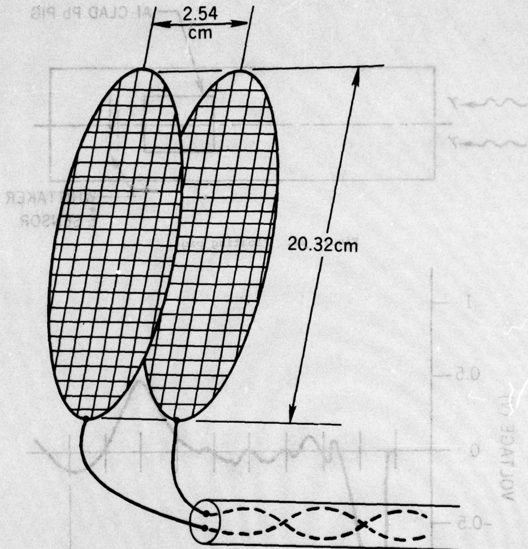
Figure 21. Whittaker \dot{E} sensor.
