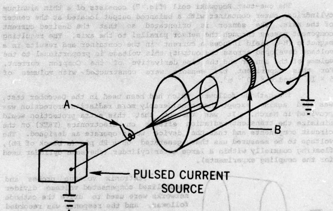
Figure 6. Bench test.
