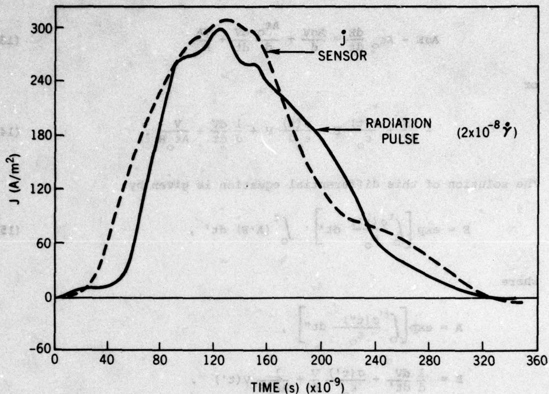
Figure 17. Compton-current time history.
