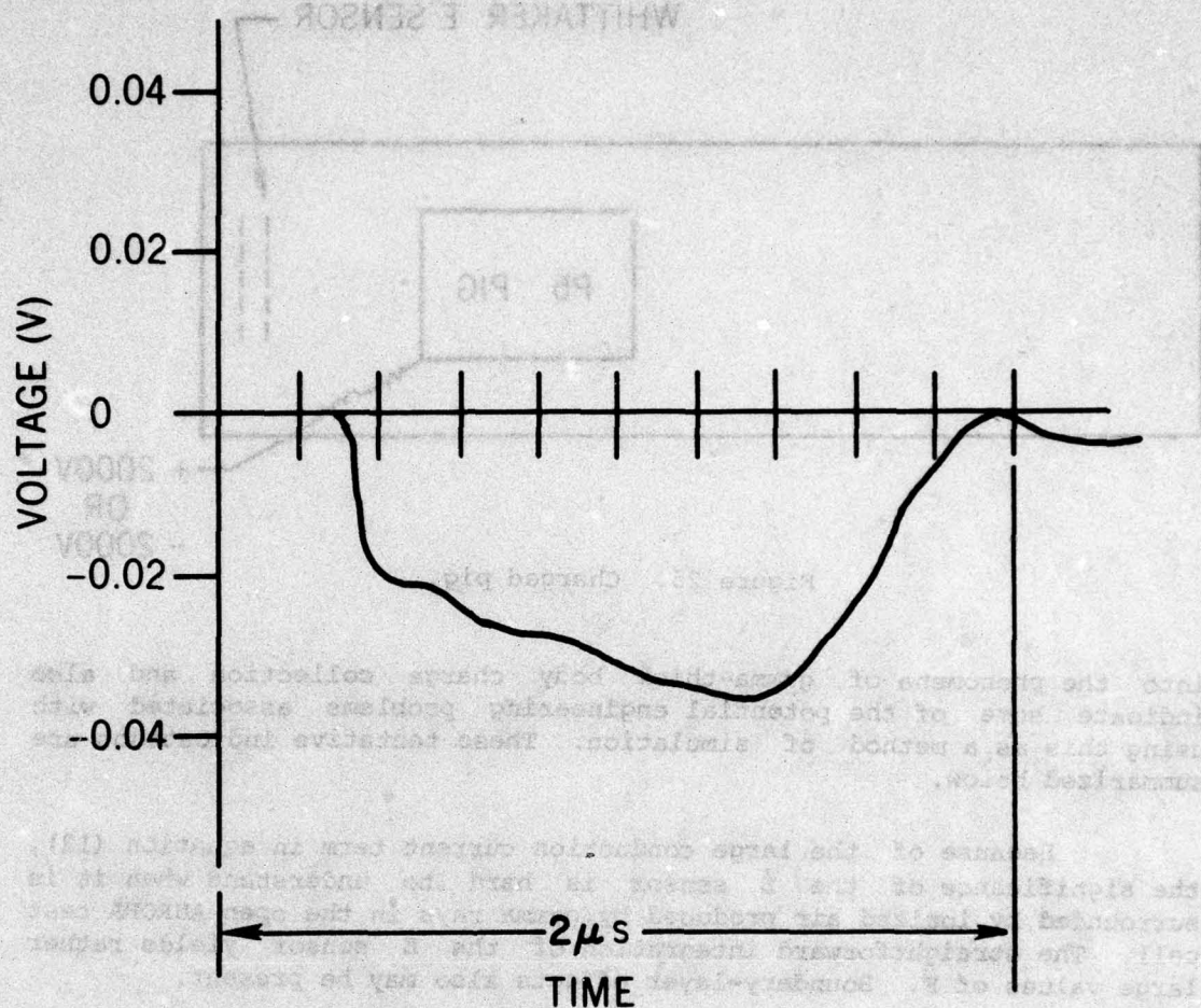
Figure 24. Integration of \vec{E} sensor response.
