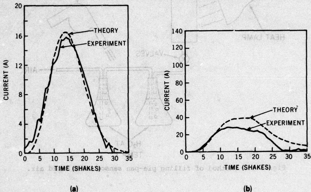
Figure 15. Pie-pan response: (a) dry air and (b) nitrogen (bias: 1000 V).
