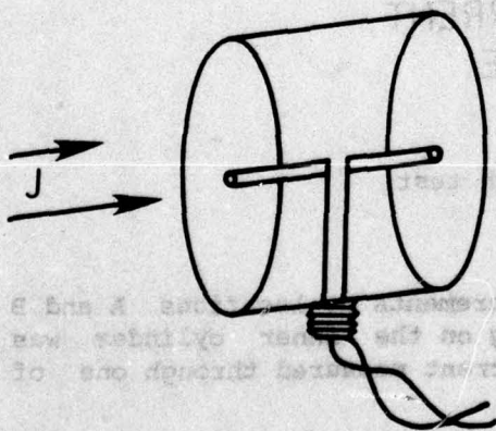
Figure 7. One-turn Rogowski coil (J sensor).
