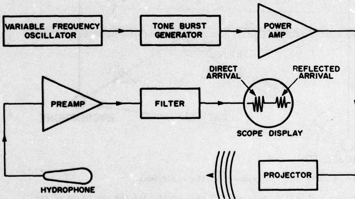
Figure 6. Block diagram of the electronics.
