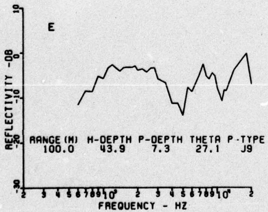
Figure 10. Reflectivity measured in Barrow Strait in April, 1972.
