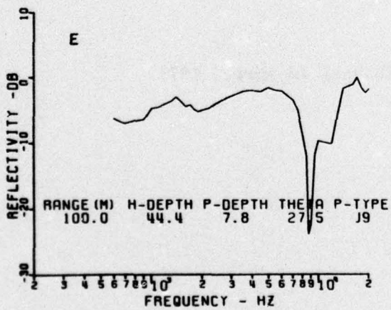
Figure 9. Reflectivity measured in Robeson Channel in April, 1972.
