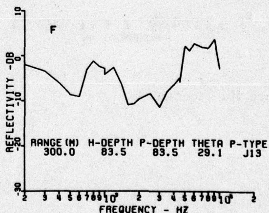
Figure 11. Reflectivity measured in Barrow Strait in April, 1973.
