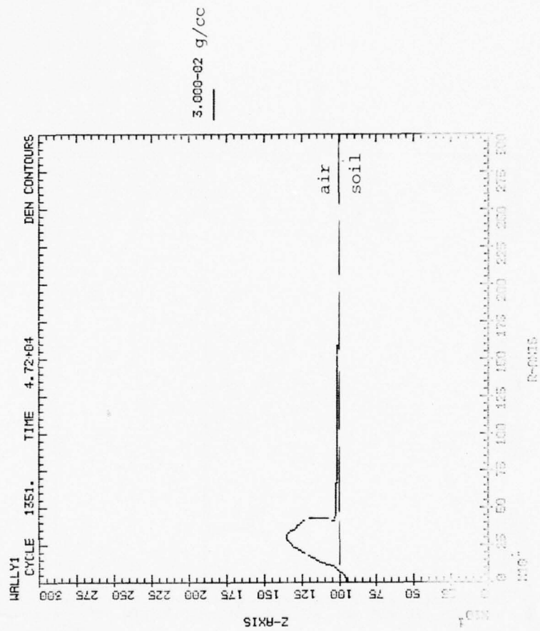
FIGURE A.15 RAD9 CALCULATION, 1-KT AT 0.5-METER DEPTH, t = 0.472 MSEC; 3 \times 10^{-2} g/cc DENSITY CONTOUR
