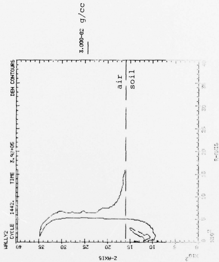
FIGURE A.34 RAD9 CALCULATION, 1-KT AT 3-METER DEPTH, t = 3.981 MSEC; 3 \times 10^{-2} g/cc DENSITY CONTOUR
