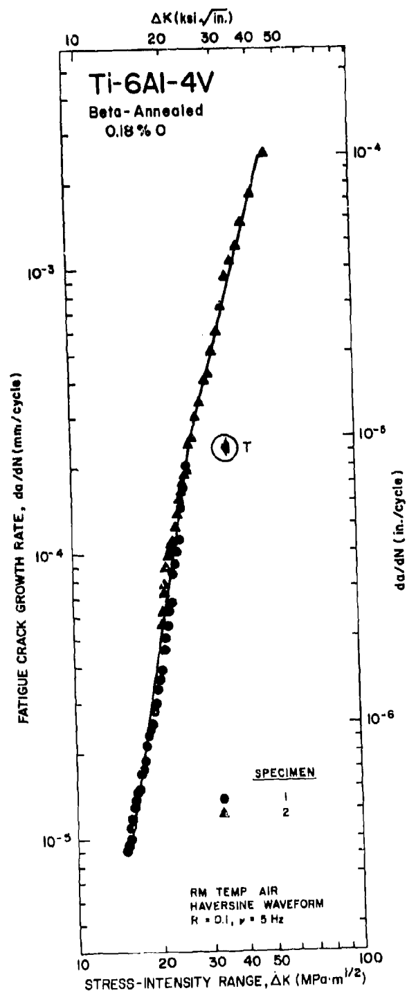
Fig. 3c — Fatigue crack growth rates for alloy 3
