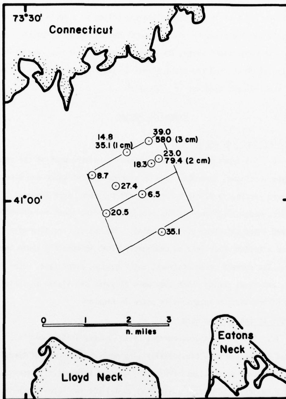
Figure 6. Location of penetroimeter stations. The bottom hardness (mb/cm, see paragraph 12) is given for each station. At stations where the hardness changed with depth in the sediment, the surficial hardness is listed above the value deeper in the sediment and the depth at which the hardness changes (in cm) is recorded
