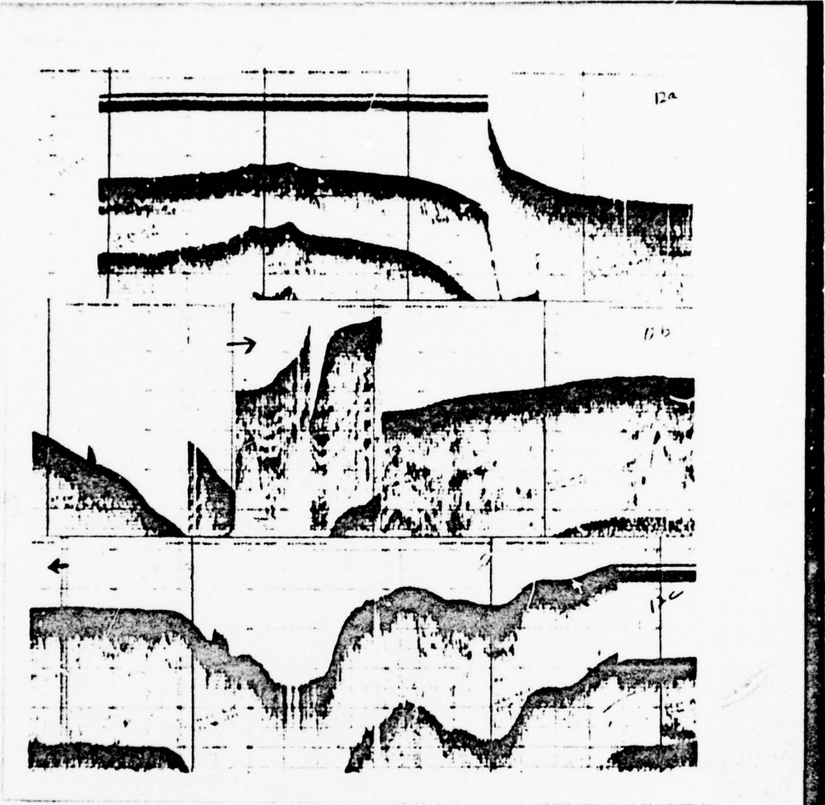
Reflection profile of track 12
