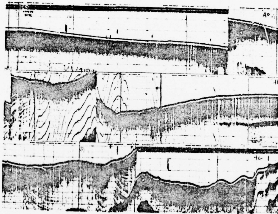
Reflection profile of track 4
