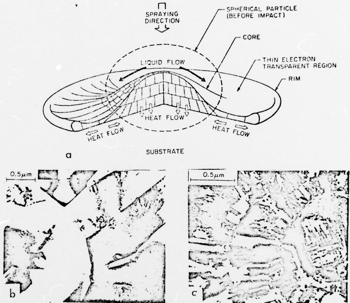
Fig. 3 - Schematic diagram of a spherical particle impinged on to a flat substrate surface (a). Transmission electron micrograph of an aluminium (b) and aluminium oxide particle (c) sprayed on to polished surfaces.
