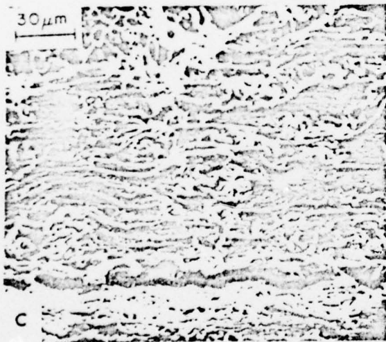
Fig. 5- Scanning electron micrographs of aluminium particles sprayed on to a flat surface (a) and grit blasted substrate (b). Cross-sectional view of sprayed aluminium (c) and Al_2O_3-TiO_2 coatings (d).
