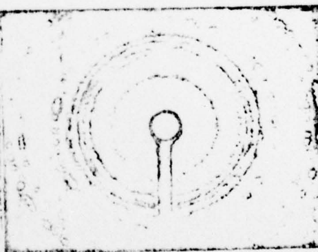
c) Electrochemically thinned polycrystalline aluminium coating and the corresponding electron diffraction pattern.
