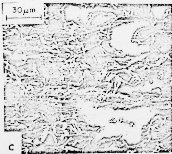
Fig. 1 - Surface of mild steel substrate grit blasted with Al_2O_3 at 45^\circ (a,b) and 90^\circ (c,d).
