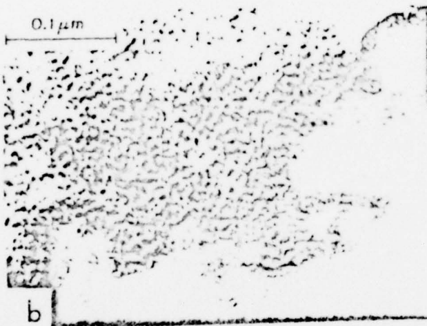
Fig. 8- TEM micrographs of plasma sprayed aluminium: a) Ultra-fine crystalline region with a diffused electron diffraction pattern. b) Same area as (a) after 15 min. under the electron beam.
