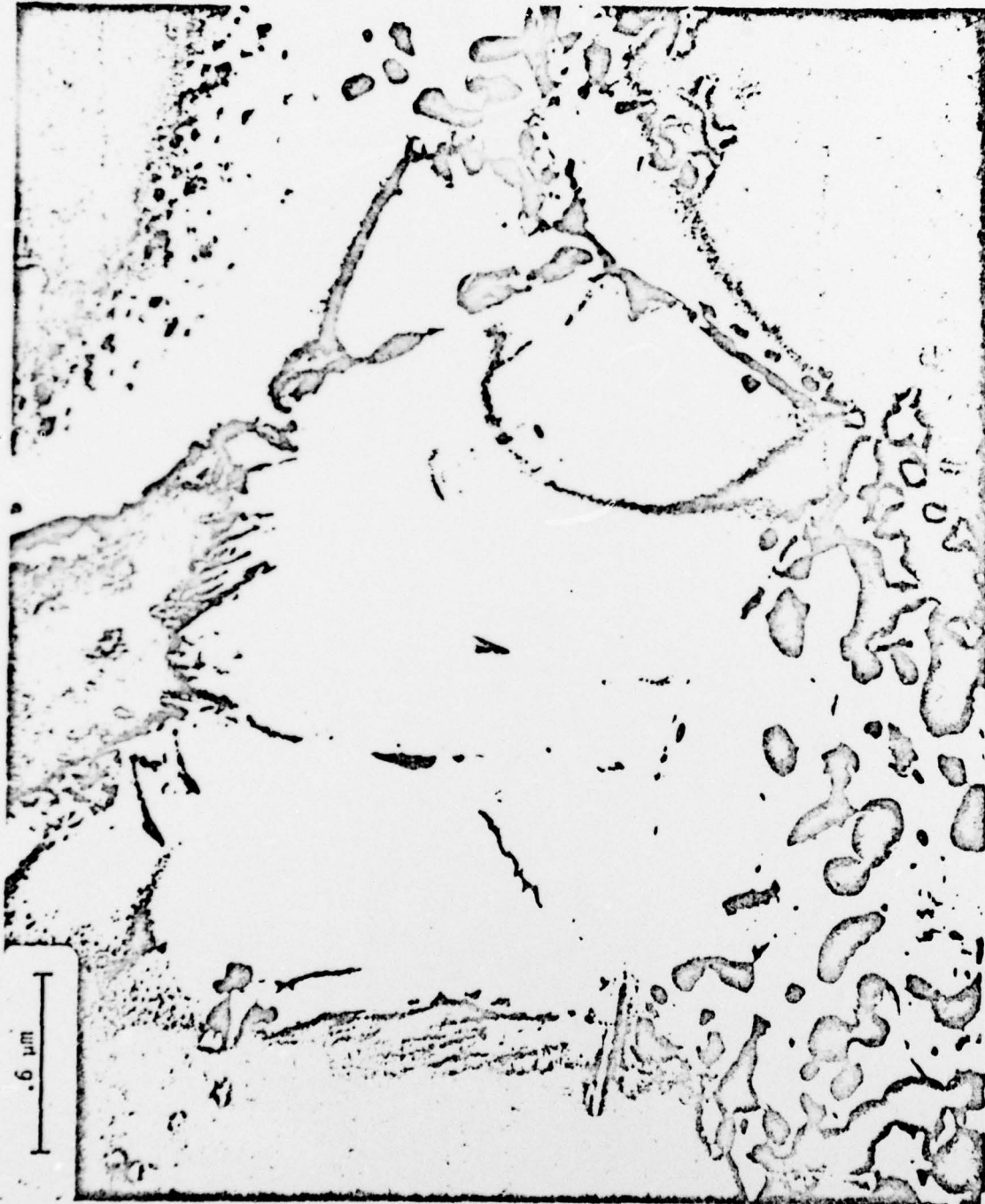
Fig. 10 - TEM micrograph of sprayed aluminum-zinc alloy showing the second phase precipitate.
