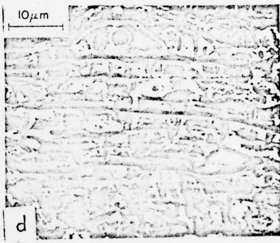
Fig. 5- Scanning electron micrographs of aluminium particles sprayed on to a flat surface (a) and grit blasted substrate (b). Cross-sectional view of sprayed aluminium (c) and Al_2O_3-TiO_2 coatings (d).
