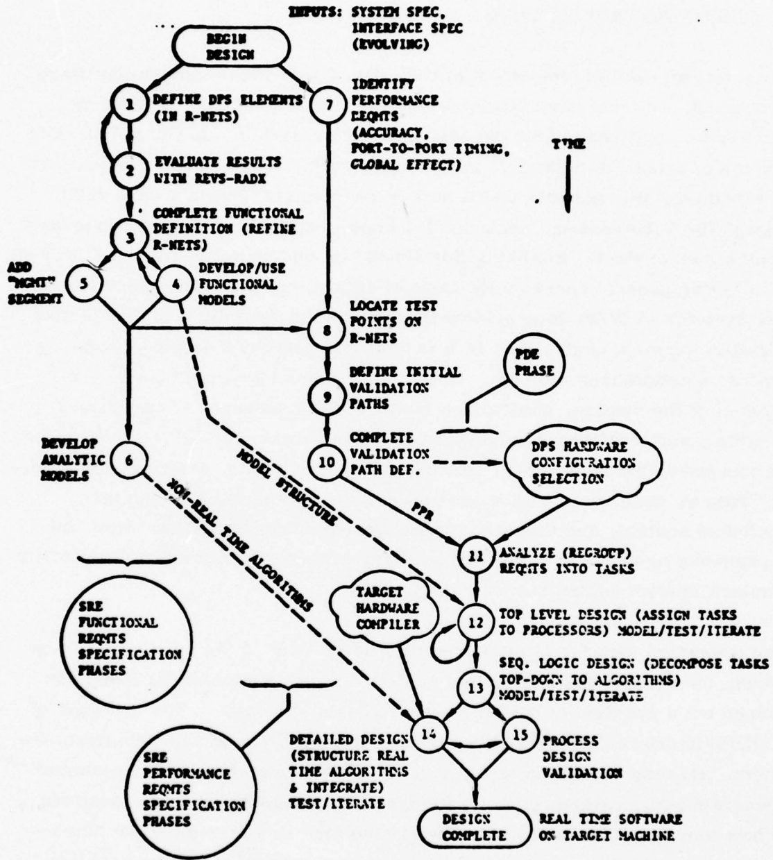
Figure 2. Fifteen Phases of SDS Design Approach
