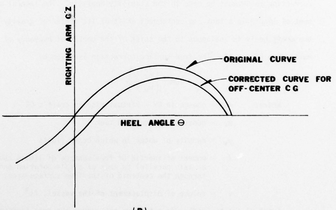
FIGURE 10 RIGHTING ARM CURVE & OFF-CENTER CORRECTION
