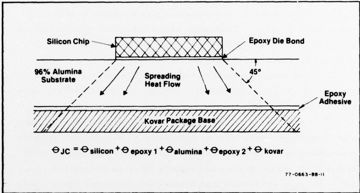
Figure 1-5. MNOS BORAM Hybrid Circuit Simplified Thermal Model
