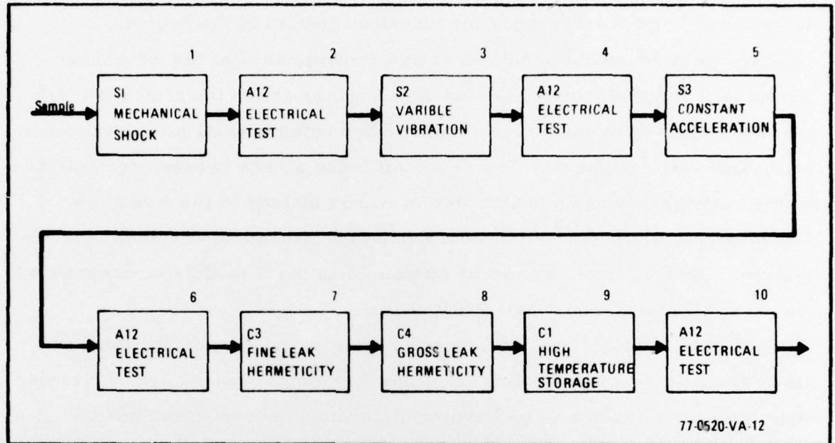
Figure 1-9. Sample Tests Required by SCS-503 for Confirmatory Sample and for Quality Conformance Inspection
