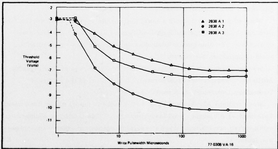
Figure 1-7. Early Write Pulse Response Measurements
