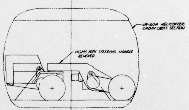
HGMS RIGGED FOR AIRLIFT IN UH-60A
