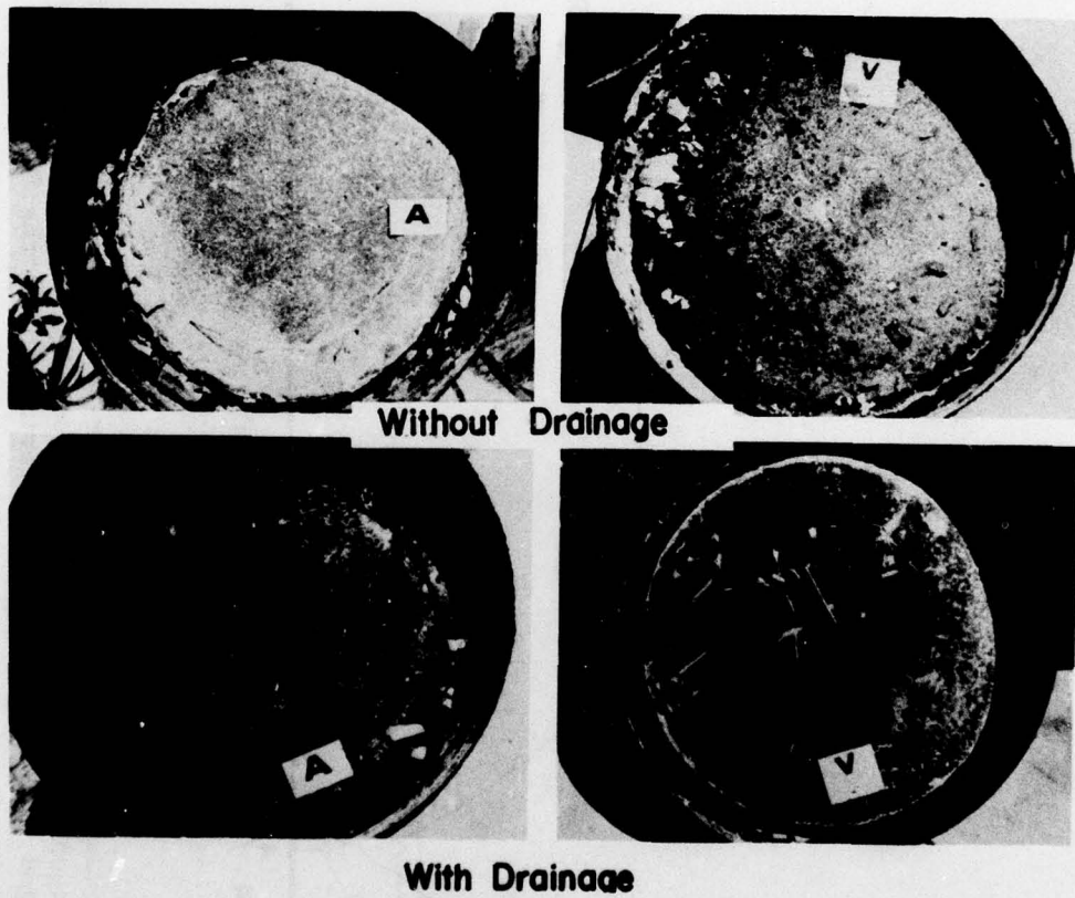
Figure 92. Containers of dredged material from Norfolk (V) and Mobile (A) after 55 days of drying
