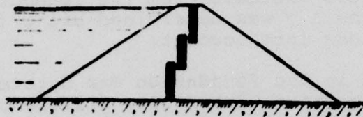
Figure 3 [sic]: Diagram of Stepped Diaphragm Core.
