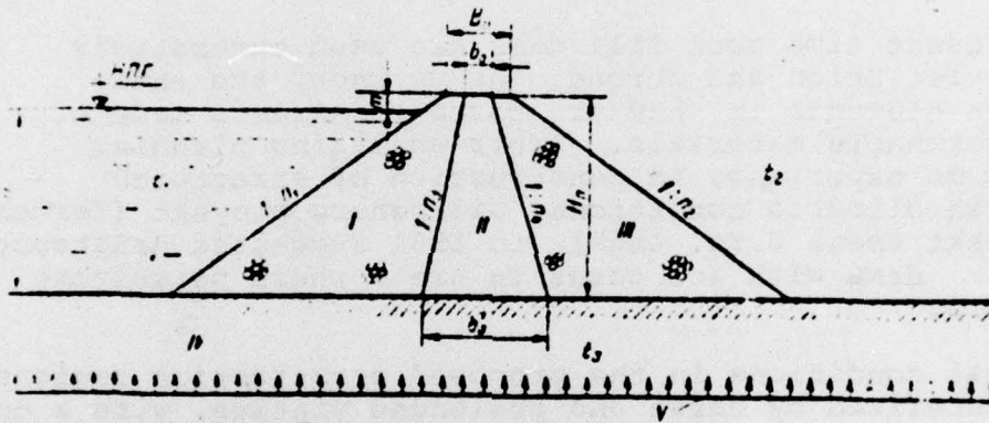
Figure I: Design Diagram of a Dam
