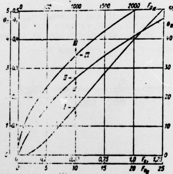
FIGURE 2. Calculation Graph to Determine Water Temperature
