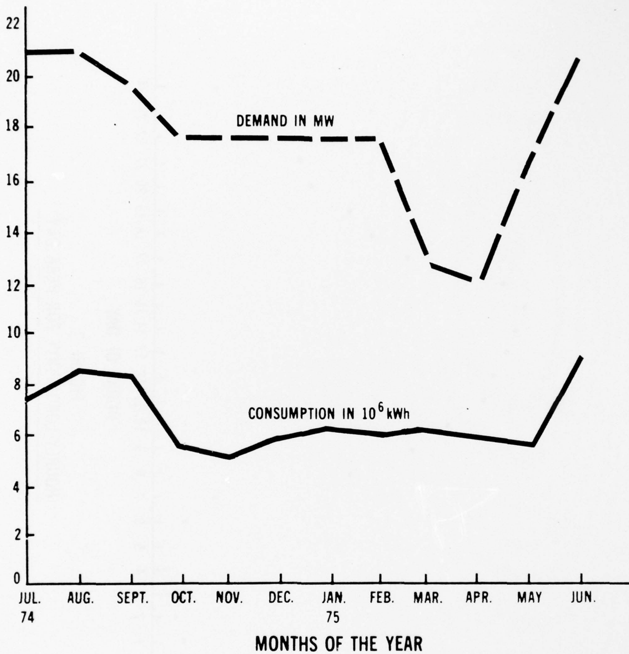
FIGURE 4 MONTHLY LOAD CURVE FOR MILITARY INSTALLATION
