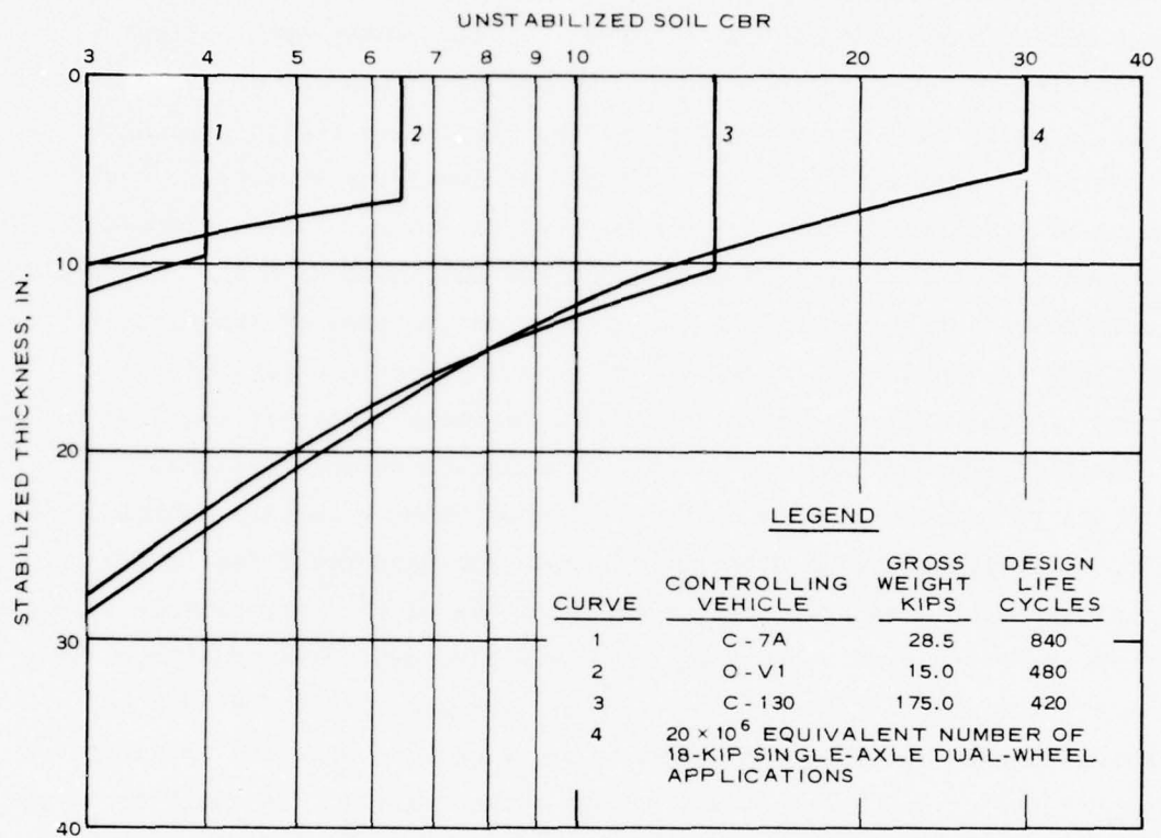
Figure 8. Road and airfield design curves for stabilized soils in forward areas
