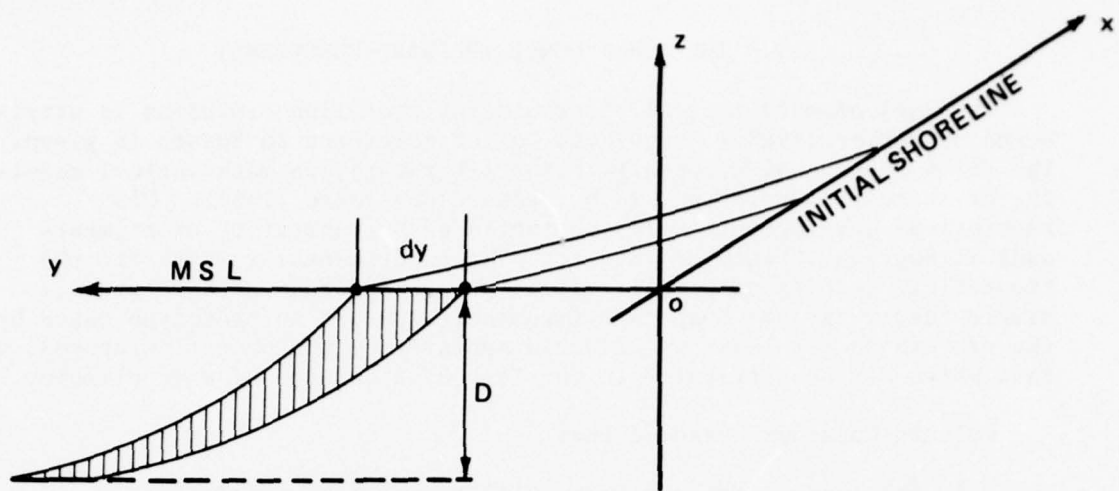
Figure 1. Beach depth definition.
