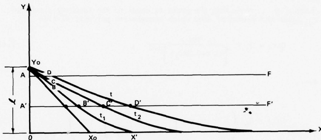
Figure 3. Successive beach profiles updrift of a groin after sand bypassing (from Le Mehaute and Brebner, 1961).
