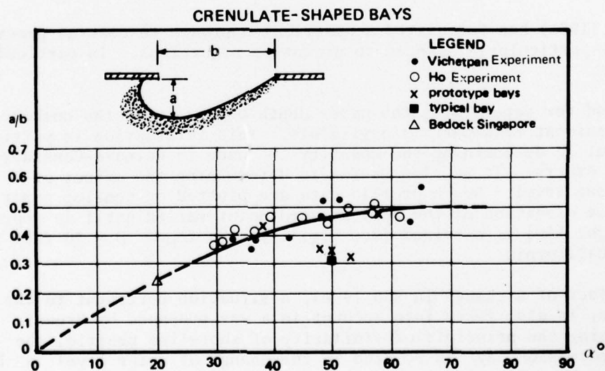
Figure 17. Indentation ratio for a range of wave obliquity (from Sylvester and Ho, 1972).
