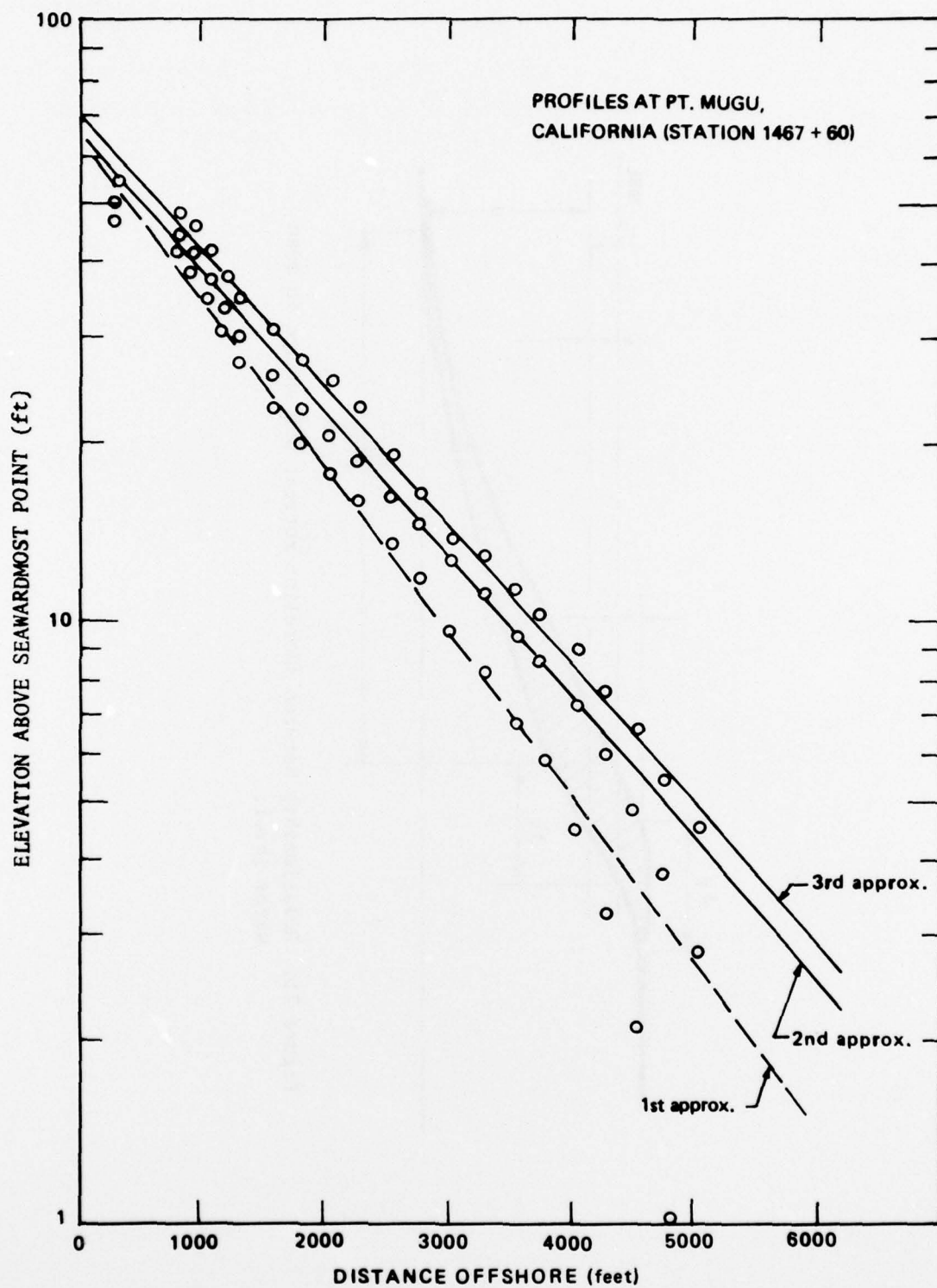
Figure 20. Semilogarithmic profiles (from Weggel, 1976).
