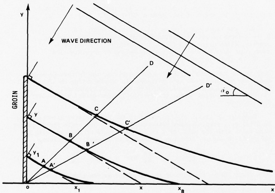
Figure 2. Successive beach profiles updrift of a long groin before bypassing (from LeMehaute and Brebner, 1961).
