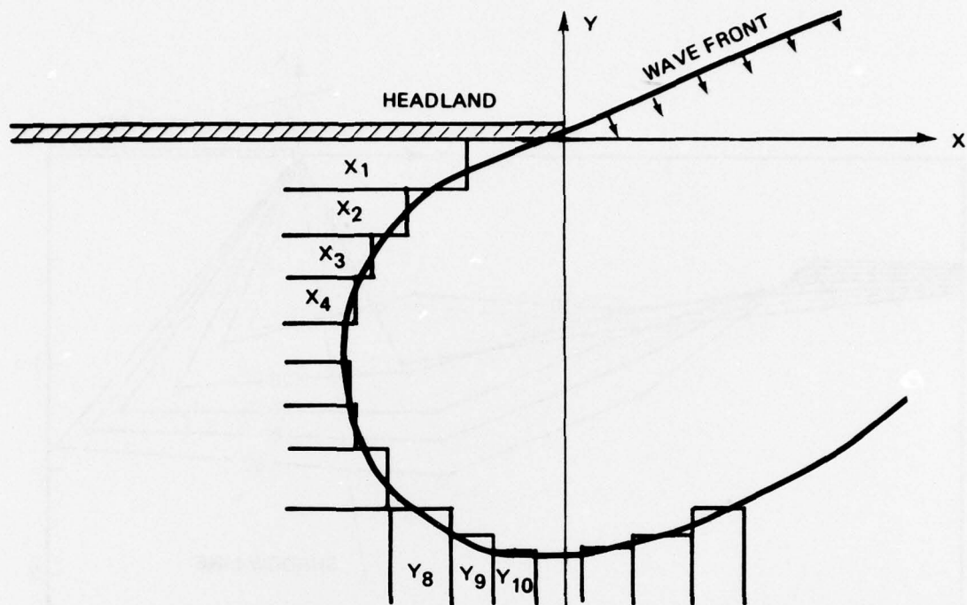
Figure 19. Orthogonal arrays for numerical scheme of hooked bay (from Rea and Komar, 1975).
