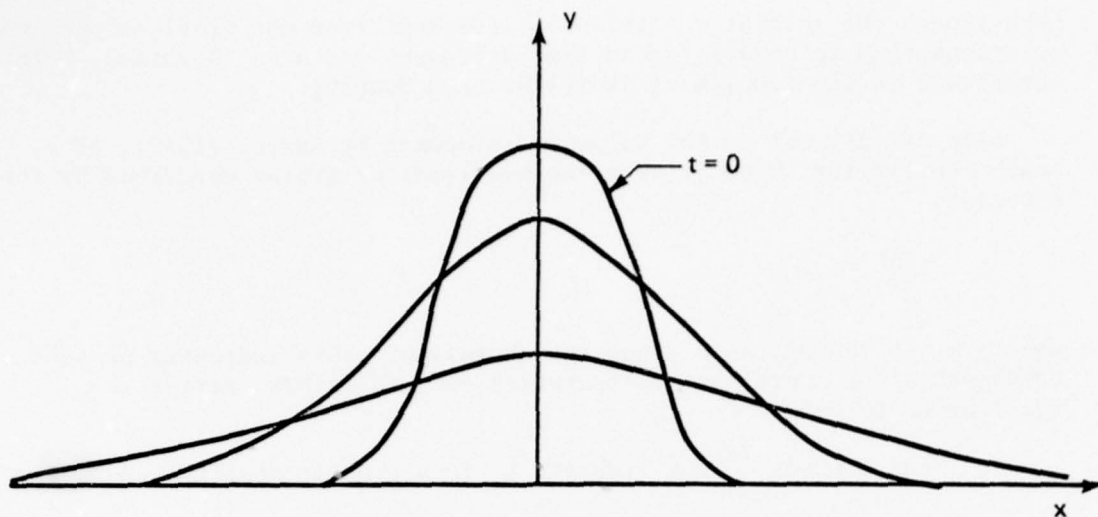
Figure 8. Spreading of sand along a shoreline due to instantaneous dumping at a point.
