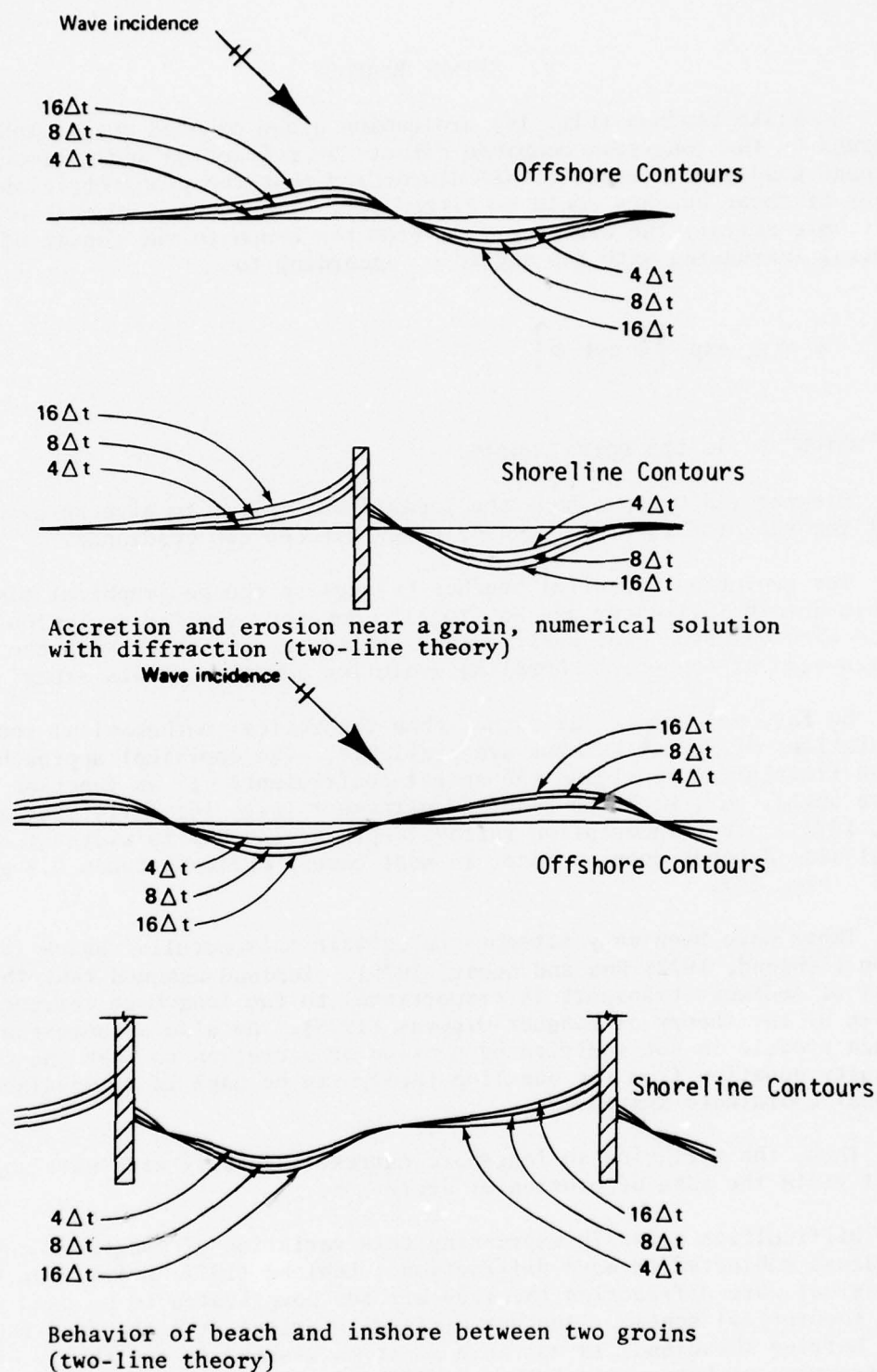
Figure 15. Effect of wave diffraction (from Bakker, 1970).
