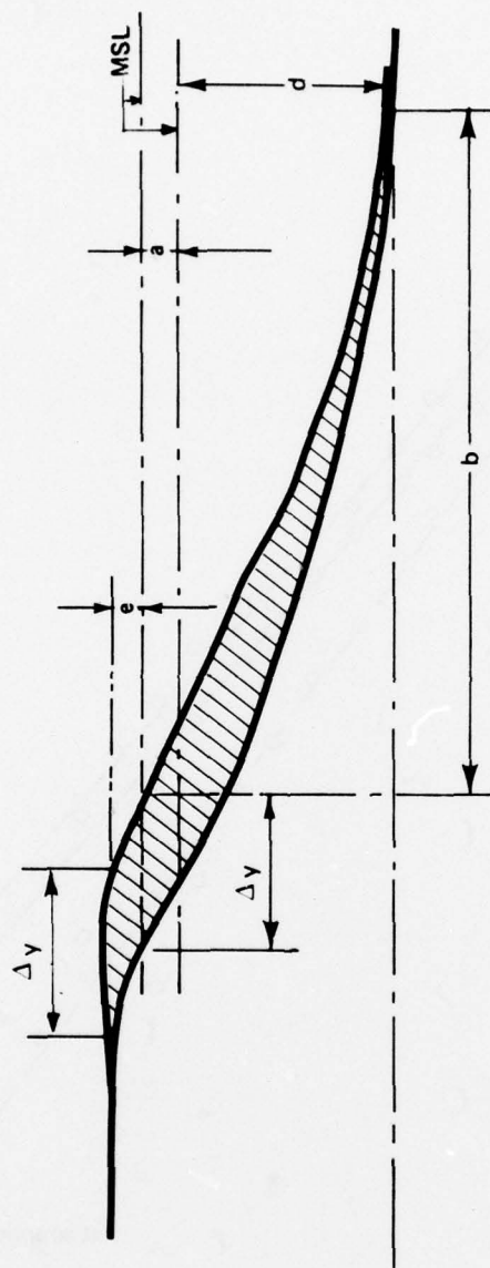
Figure 21. Relationship between shoreline retreat and change in mean water level.
