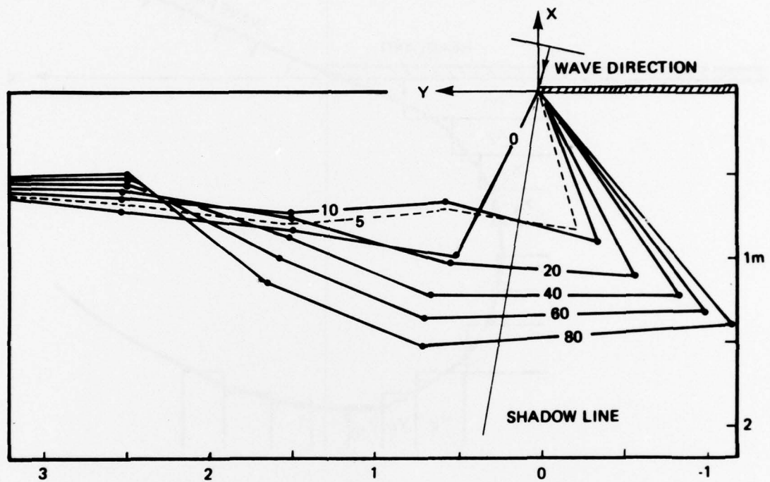
Figure 18. Orthogonal arrays for numerical scheme of hooked bay (from Leblond, 1972).
