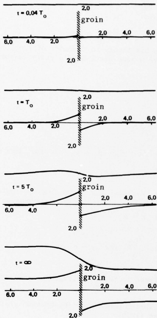
Figure 14. Evolution of shoreline and offshore beach limit near a groin (from Bakker, 1968b).
