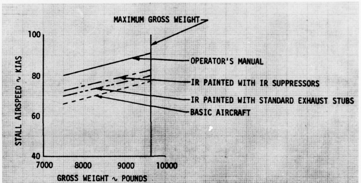
Figure A. Stall Airspeed Variation With Modification - Cruise Configuration.
