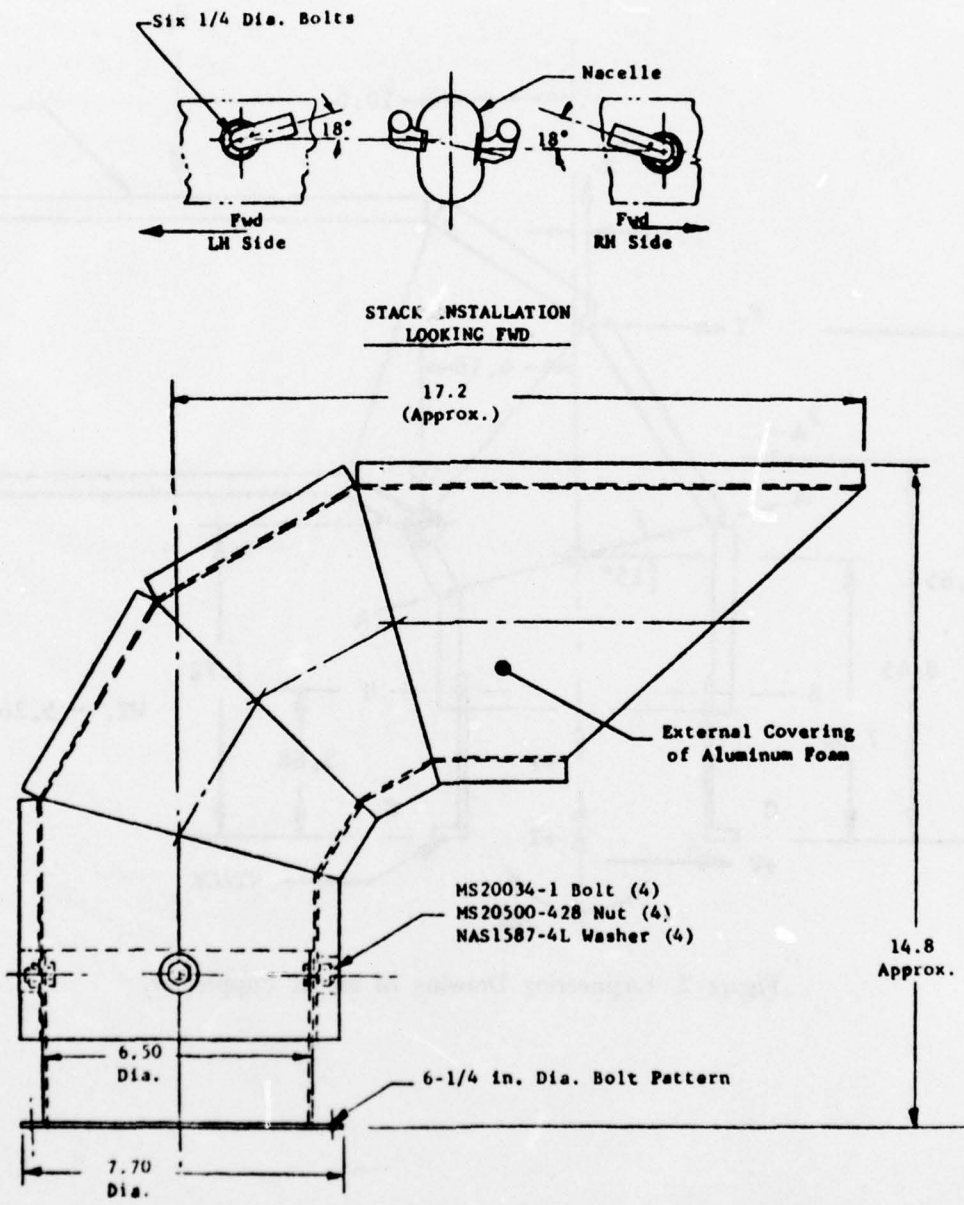
Figure 3. IR Suppressor Detail Drawings.
