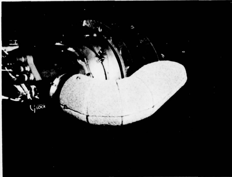
Photo 8. Front View - Right U-21A Engine (No. 2) With IR Suppressors Installed.
