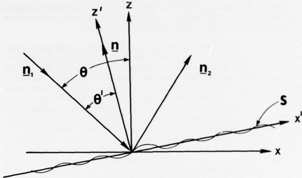
Figure 1. Scattering Geometry
