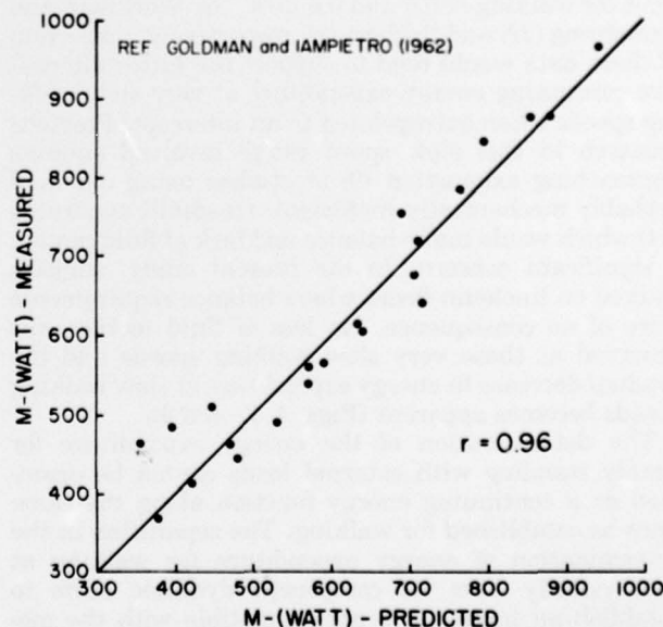
FIG. 4. Measured and predicted energy expenditure for walking at various speeds ( 0.7\text{--}1.8\text{ m}\cdot\text{s}^{-1} ), external loads ( 10\text{--}30\text{ kg} ), and grade elevations ( 3\text{--}9\% ). Reference is to work by Goldman and Iampietro (10).
