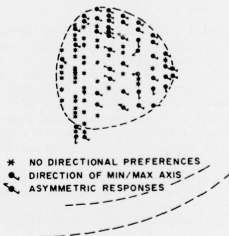
Figure 3. Visual response patterns seen in 10 selected electrode tracks are plotted against a diagram of a sagittal section through the center of the nucleus rotundus. The neurones were classified according to their responses to different directions of stimulus movement as described in Figures 1 and 2. There is a clear tendency for units without directional selectivity or preferences to cluster in the posterior third of rotundus.
