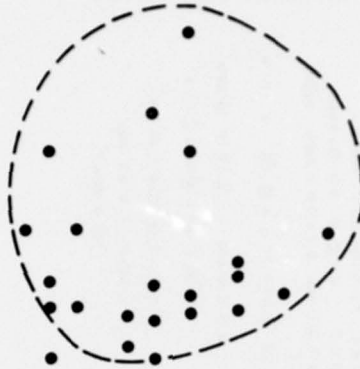
Figure 5. Responses to single nonmoving flashes of light, spots or whole field, are seldom seen in rotundus. In this diagram we have condensed results from 20 electrode tracks. Units responding to flash tend to cluster in the ventral third of the nucleus.
