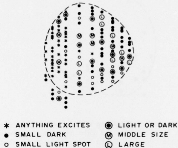
Figure 4. Responses from another set of 10 tracks are plotted as before. The responses are categorized according to size preferences (Figure 1, C and D). The units nonselective for size seem to cluster in the posterior third of rotundus.
