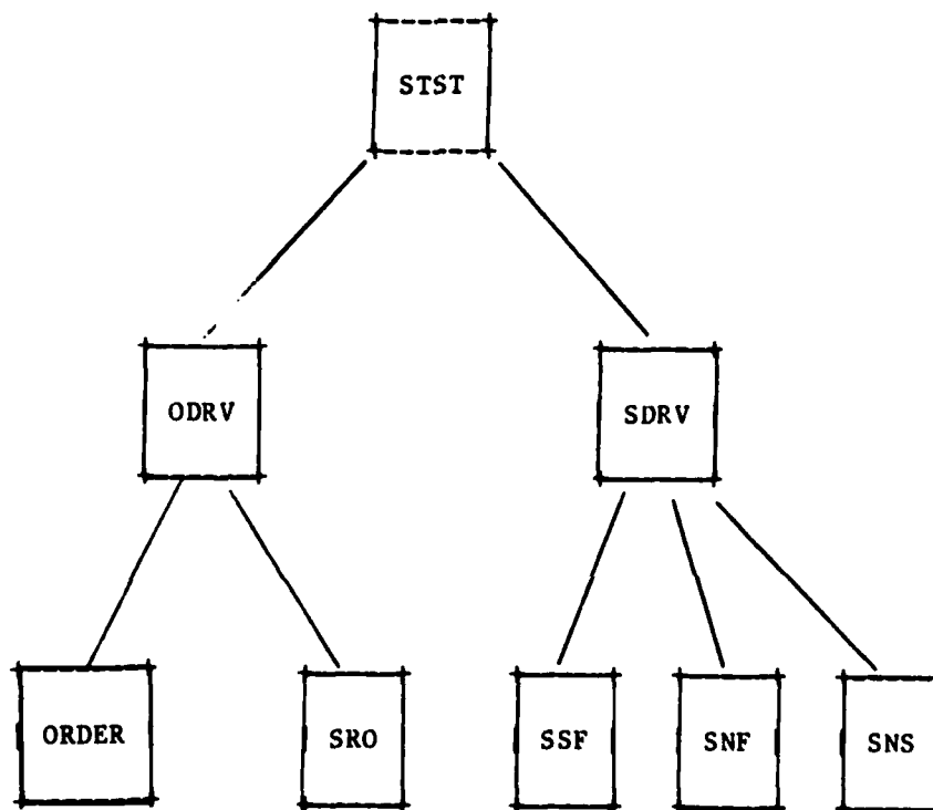
Figure 1: A schematic overview of the sparse symmetric matrix package
