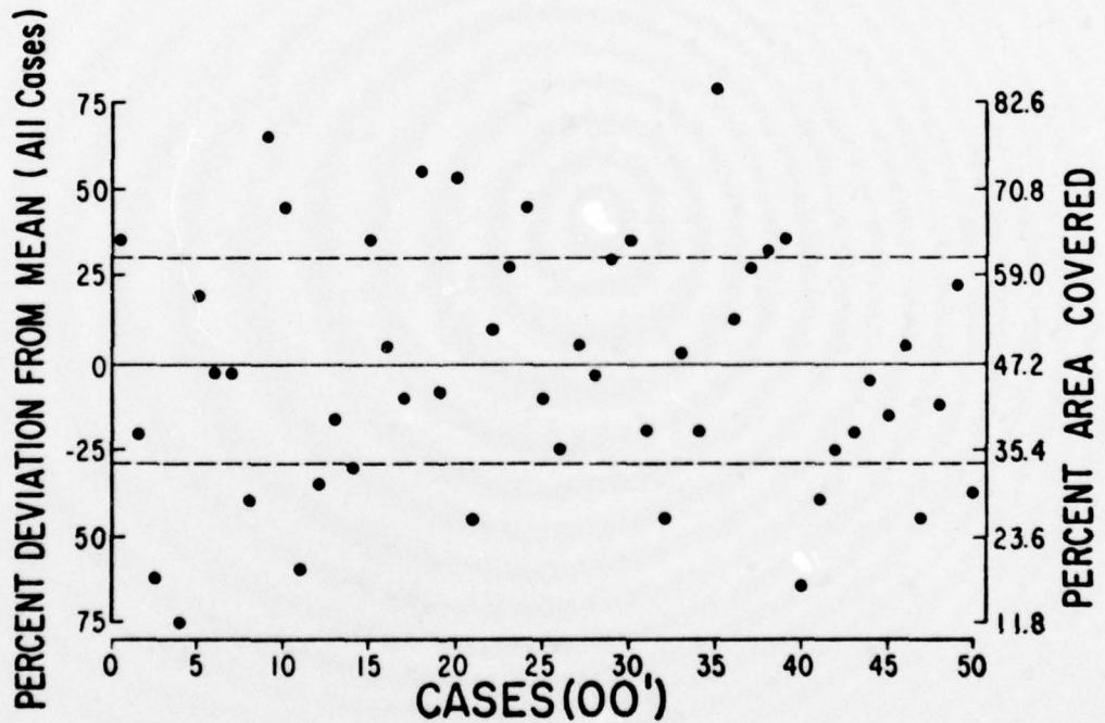
Fig. 28. A representative sample ( \sim 40\% ) of the daily variability displayed by total cirrus within the 3 \times 3 area ( r \sim 4.2^\circ ) for the developing (ES1) and non-developing (00') disturbances. The dashed lines represent the mean of plotted cirrus samples above and below the case mean values.
