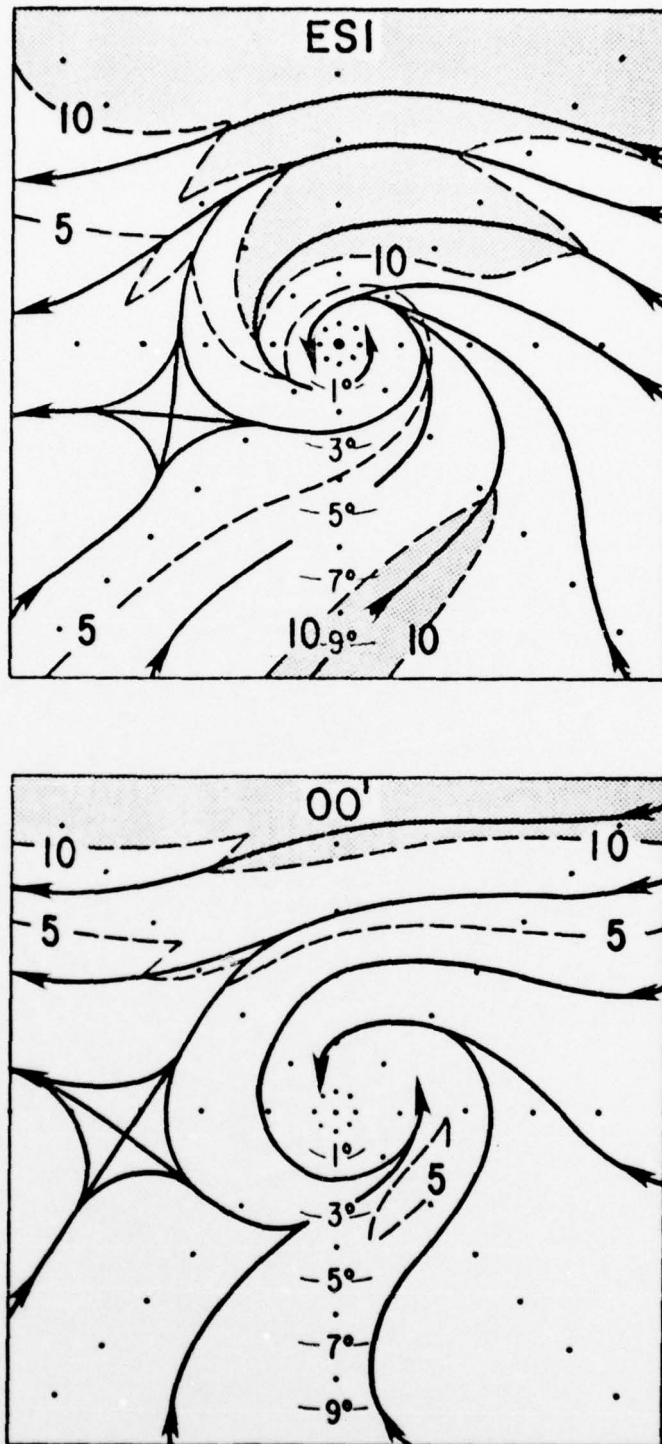
Fig. 21. Average isotach ( \text{m s}^{-1} ) and streamline analysis for the developing (ESI - above) and non-developing (00' - below) disturbances at 950 mb.
