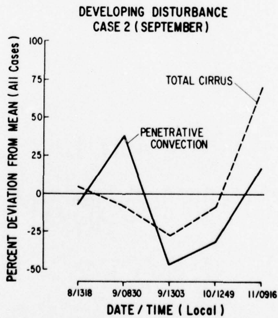
Fig. 32. Daily variability of penetrative convection and total cirrus within the 3x3 area ( r \sim 4.2^\circ ) of developing disturbance case (2) corresponding to Fig. 31.
