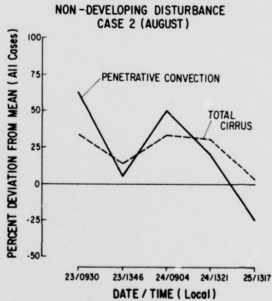
Fig. 36. Daily variability of penetrative convection and total cirrus within the 3x3 area ( r \sim 4.2^\circ ) of non-developing disturbance case (2) corresponding to Fig. 35.
