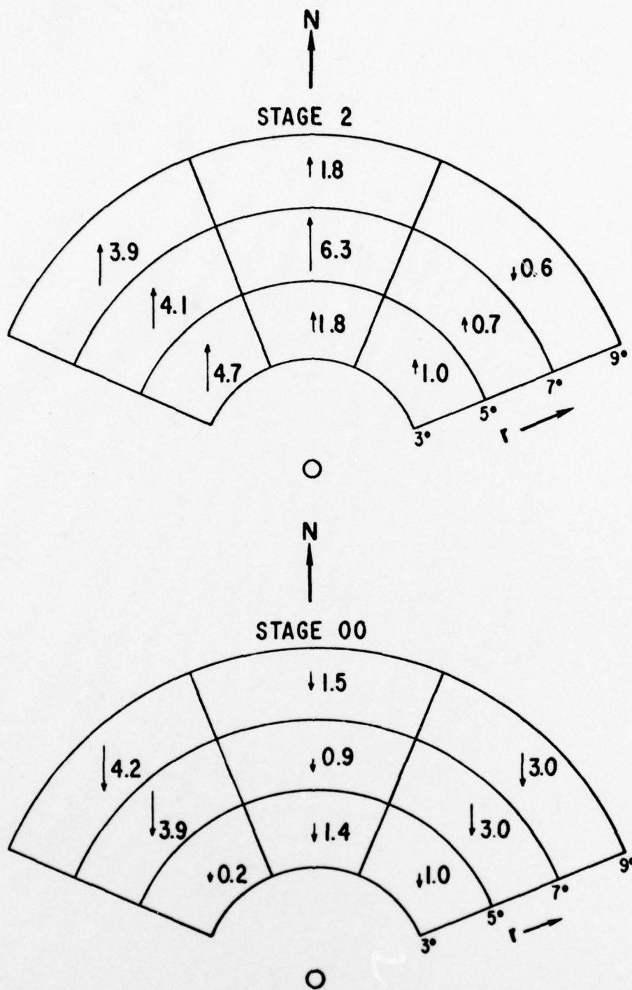
Fig. 25. Composited 200 mb meridional ( v ) component of the wind ( \text{m s}^{-1} ) from Zehr's (1976) developing (Stage 2) and non-developing (Stage 00) rawinsonde composites. Each octant-belt represents an average of about 30 rawinsonde reports.
