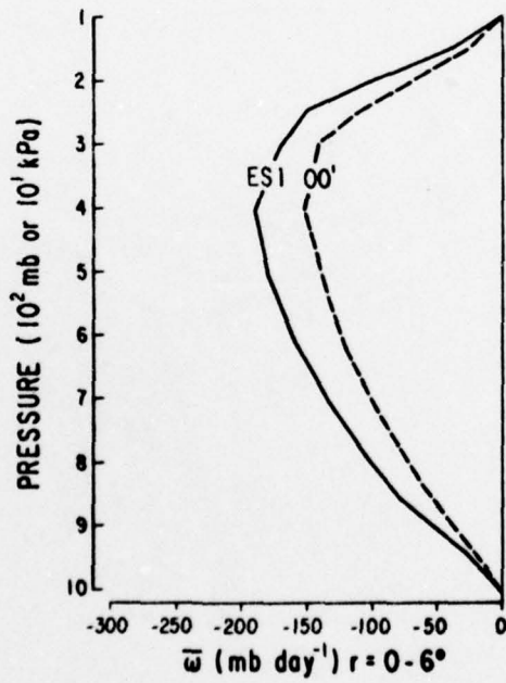
Fig. 14. Same as Fig. 13, except r = 0-6^\circ .
