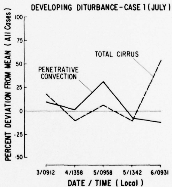
Fig. 30. Daily variability of penetrative convection and total cirrus within the 3 \times 3 area ( r \sim 4.2^\circ ) of developing disturbance case (1) corresponding to Fig. 29.
