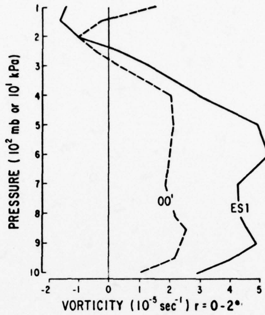
Fig. 16. Mean relative vorticity within area r = 0-2^\circ for the developing (ES1) and non-developing (00') disturbances.
