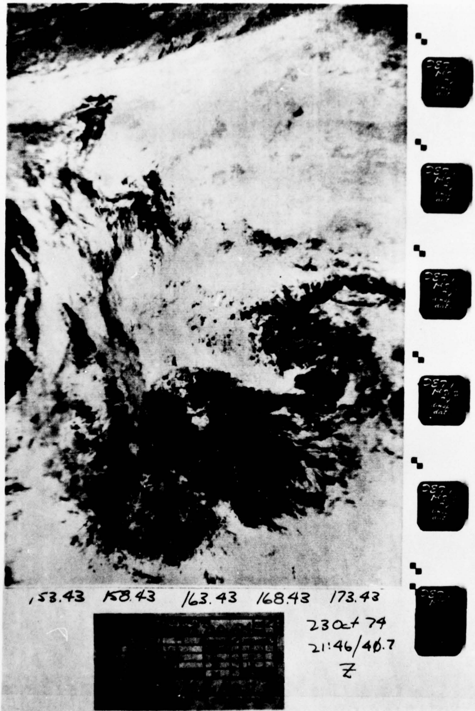
Fig. 1b. An example of a DMSP infrared film transparency which corresponds directly to Fig. 1a. Longitude and time of nodal crossing are listed in legend (i.e., 163.4^{\circ}\text{E} and 21:46 GMT).
