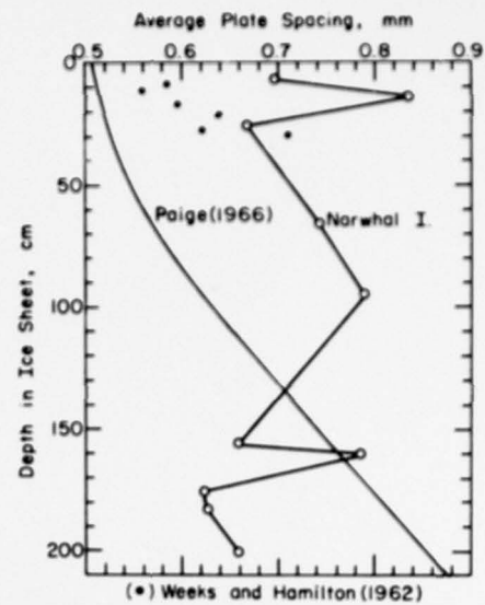
Figure 4. Subcrystal plate width versus depth of ice at Narwhal Island. Curve (Paige 1966) was generalized from profiles obtained from several different locations in McMurdo Sound, Antarctica.
