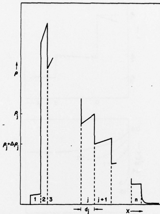
Fig. 2 — Schematic quasi-steady density profile of layered, inhomogeneous, laser-driven target consisting of n strata of distinct fluids. Jump in density from layer j to j+1 is \Delta\rho_j .
