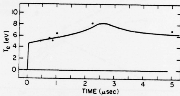
Fig. 11 — History of the electron temperature after beam injection. T_e is obtained from H\beta line-to-continuum studies. The points show Thomson scattering data, each data point being the average of three shots.
