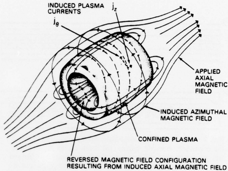
Fig. 1 — Rotating relativistic electron beam induced axial ( j_{z-net} ) and azimuthal ( j_{\theta-net} ) plasma currents and the resultant azimuthal (toroidal) field, B_\theta , and axial (poloidal) field B_z , respectively
