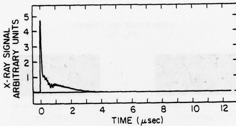
Fig. 7 — Temporal dependence of hard x-ray emission from a 1 mm diameter tungsten wire placed across the drift tube
