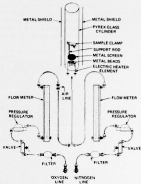
Figure 1. Schematic of apparatus.
