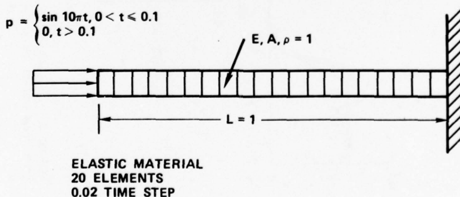
FIGURE 1. One-Dimensional Rod Geometry.
