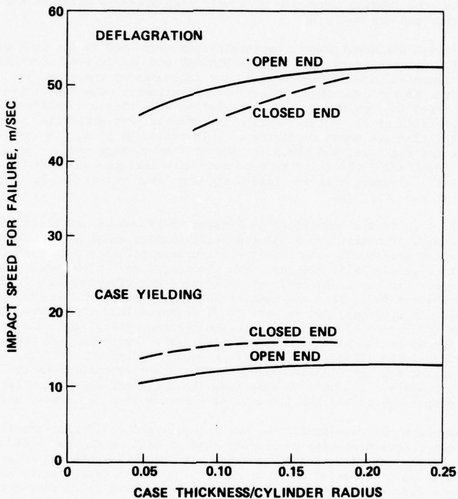
FIGURE 14. Effect of Wall Thickness on Failure Speed.
