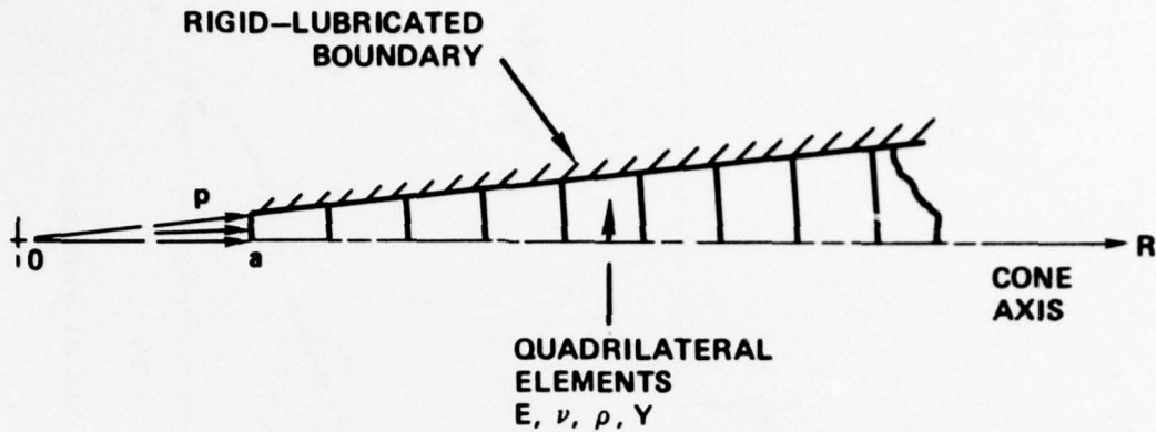
FIGURE 21. Geometry of Spherical Cavity Model.
