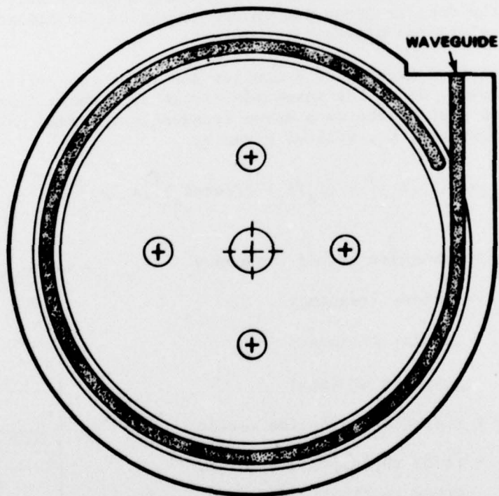
FIGURE 1. Basic Design of a Waveguide Doppler Generator.
