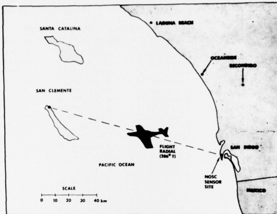
Figure 4. Geometrical configuration for NOSC aircraft spectrometer operation.
