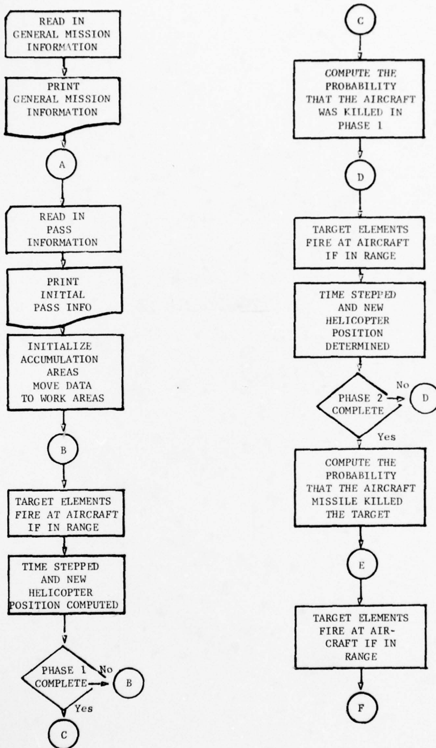
Figure IV-8-- HOVARM Flow Chart
