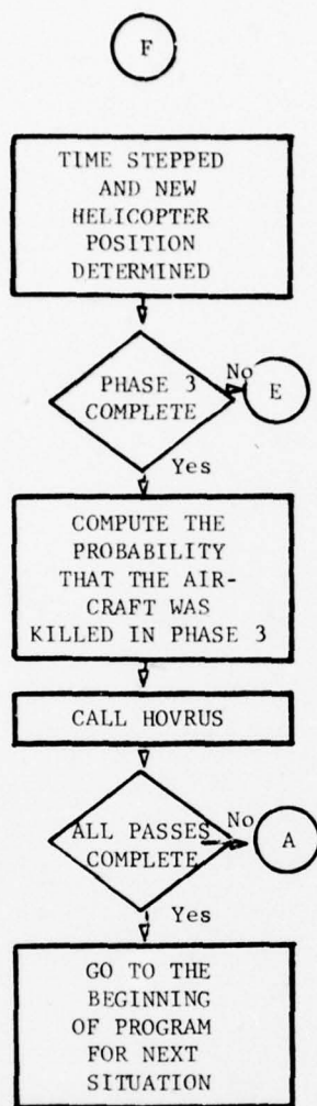
Figure IV-8--HOVARM Flow Chart--Continued
