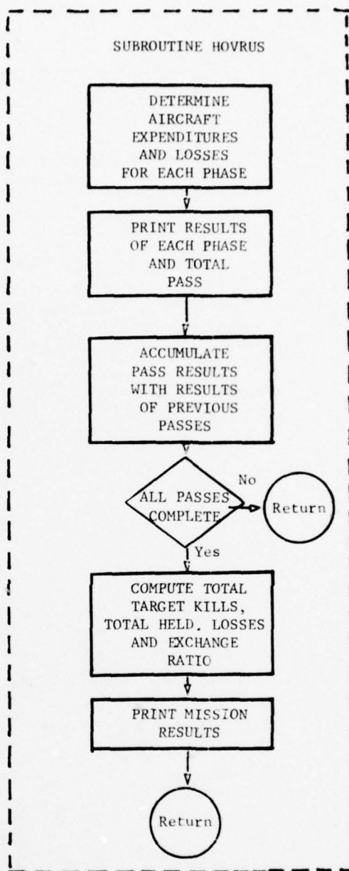
Figure IV-8--HOVARM Flow Chart--Continued
