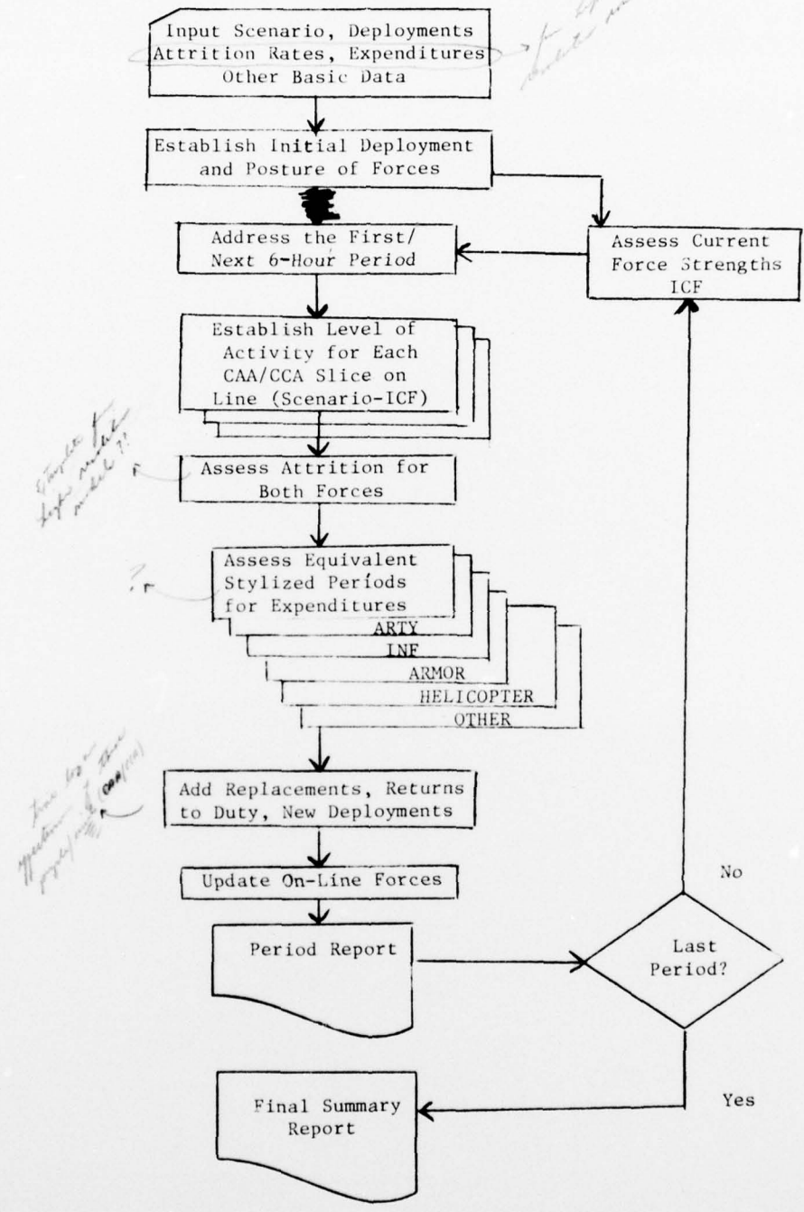
Figure IV-18--Logic Flow of Theater Rates Model
