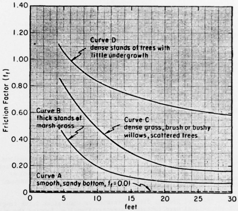
Figure 13. Bottom-friction factors.
