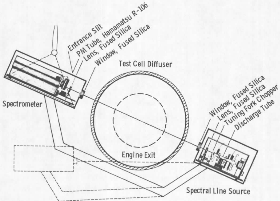
Figure 1. Diagram of installation of spectral absorption apparatus in Propulsion Development Test Cell (J-2) for NO and NO 2 concentration measurements in exhaust of F101 engine.
