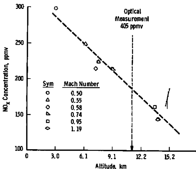
Figure 6. Results of probe-measured values of \text{NO}_x concentration versus altitude at centerline of jet engine exhaust at intermediate power.
