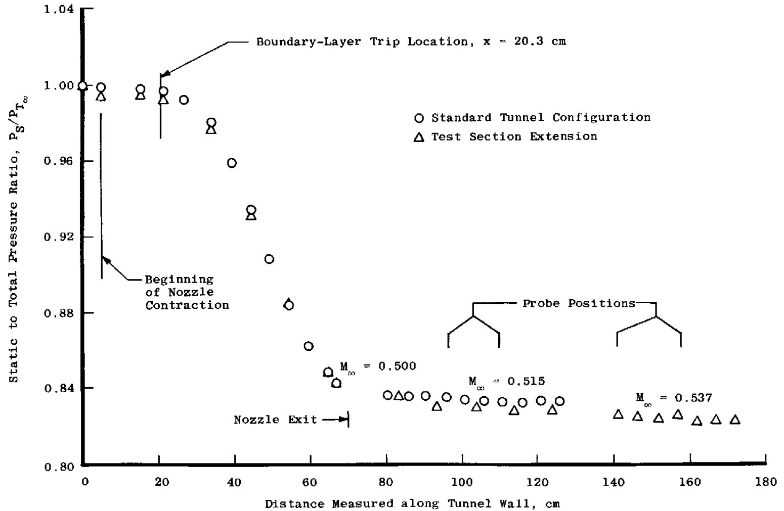
Figure 6. Static pressure gradient in the ART at M = 0.5 .
