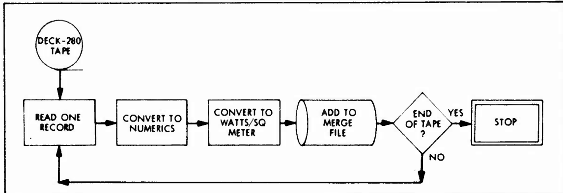
FIGURE 5-3. DECK280 COMPUTER PROGRAM
