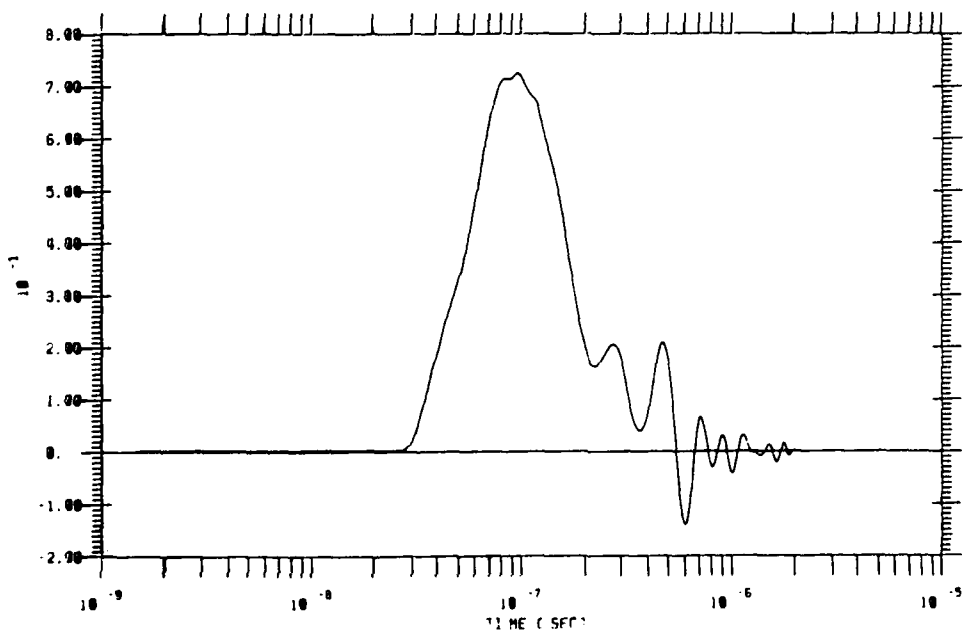
Figure 32b. V_{OC} for Measured Amplitude and Calculated Phase (Horizontal Polarization)
