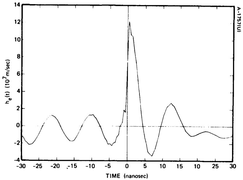
Figure 1a. h_e(t) for the Vertically Polarized Data
