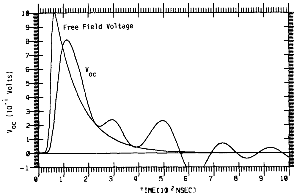
Figure 16b. Open Circuit Voltage for Horizontal Case 2 Electric Field (1 \mu sec)
