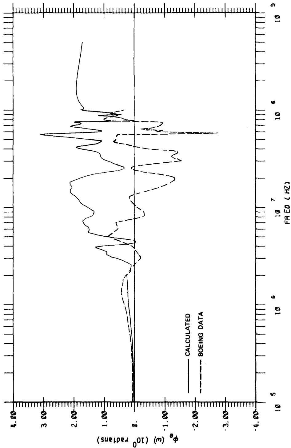
Figure 7. Phase of h_e(\omega) for a Horizontal Electric Field
