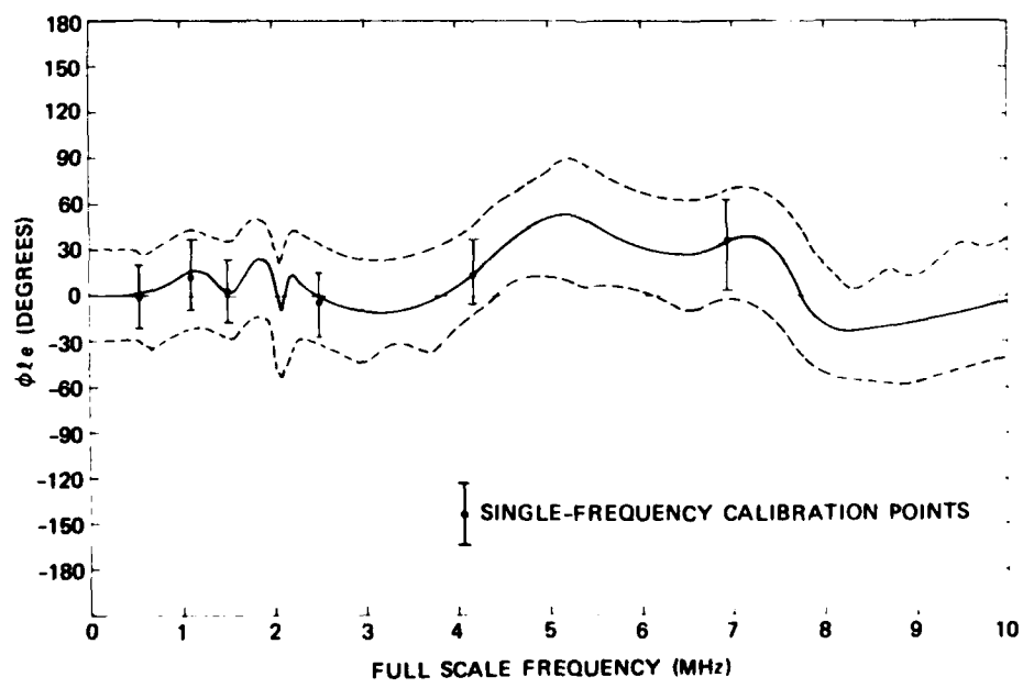
Figure 26 b. Effective Length Phase Horizontal Polarization (Final)
