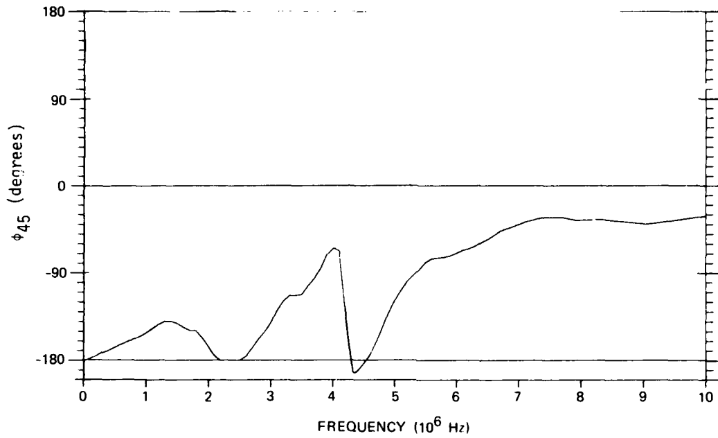
Figure 34a. 45^\circ Polarization Calculated Phase
