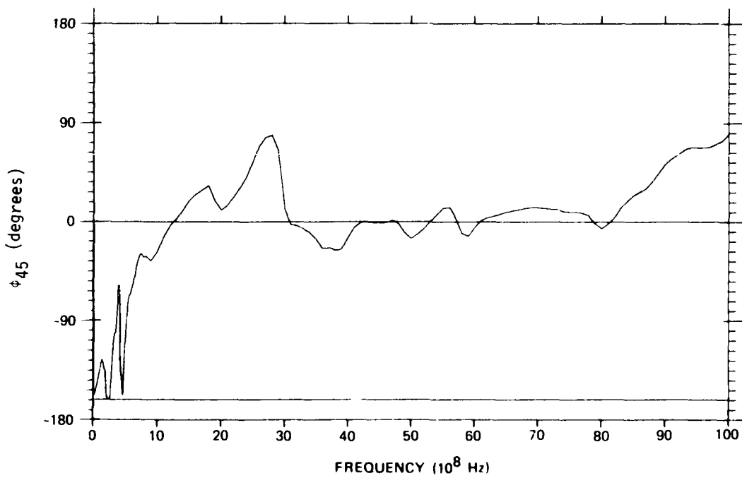
Figure 34b. 45^\circ Polarization Calculated Phase
