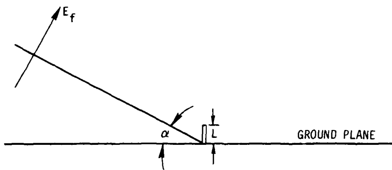
Figure 36. Incident Field on a Monopole Antenna
