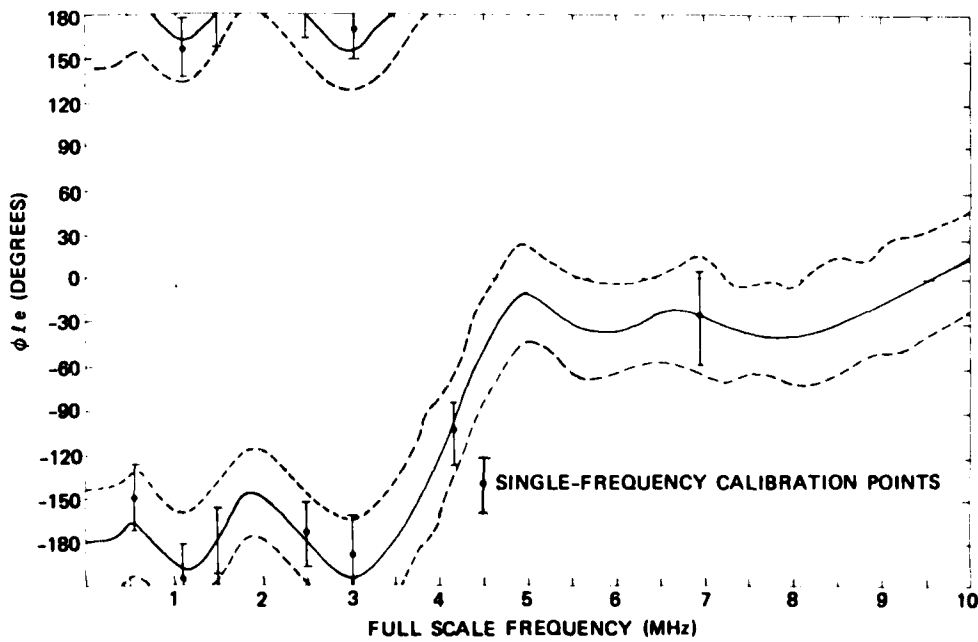
Figure 27b. Effective Length Phase Vertical Polarization (Final)
