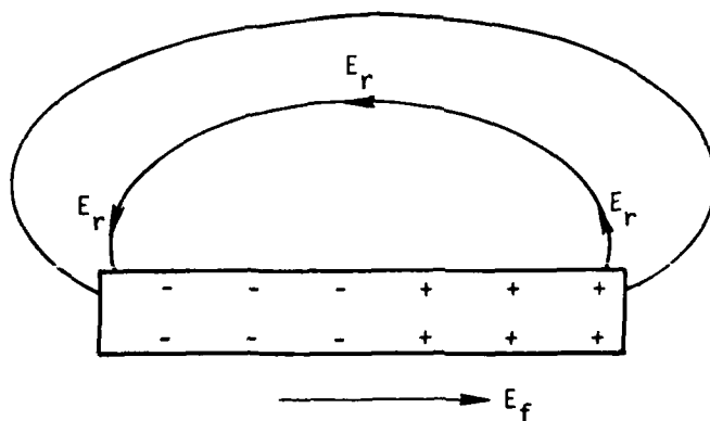
Figure 39. Electrostatic Field from a Finite Cylinder in a Horizontal Field
