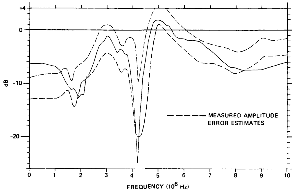
Figure 33a. 45° Polarization Calculated Amplitude (10 MHz)
