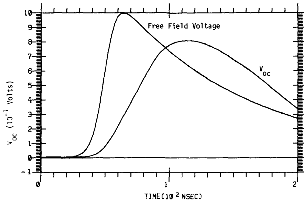
Figure 16a. Open Circuit Voltage for Horizontal Case 2 Electric Field (200 nsec)
