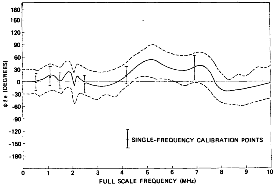
Figure 26a. Effective Length Phase Horizontal Polarization (Preliminary)
