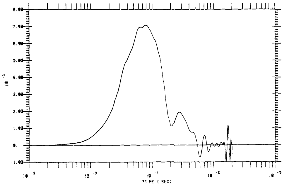
Figure 32a. V_{OC} for Measured Effective Height (Horizontal Polarization)
