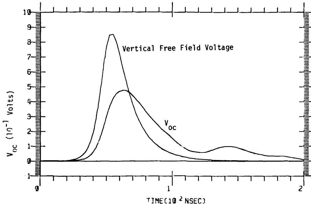
Figure 17a. Open Circuit Voltage for 30° Polarized Case 1 Electric Field (200 nsec)
