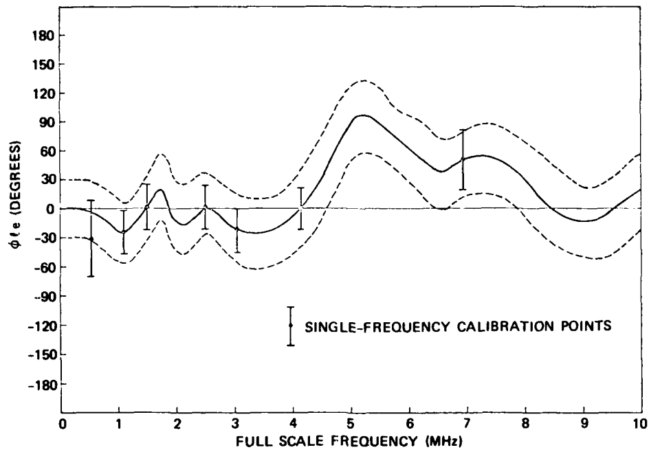
Figure 28a. Effective Length 45 Degree Polarization (Preliminary)
