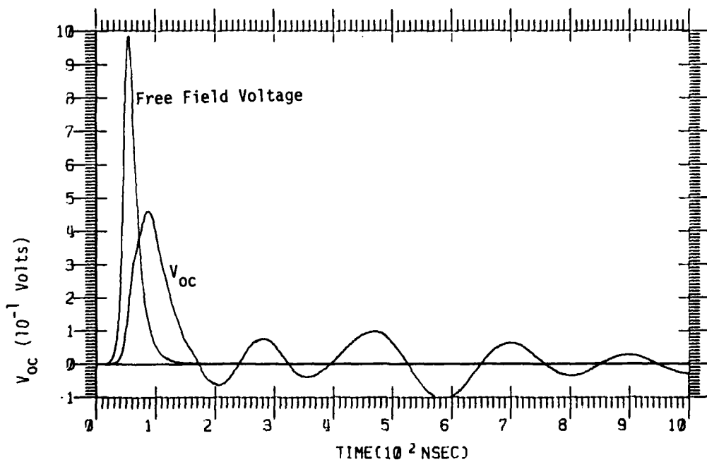
Figure 15b. Open Circuit Voltage for Horizontal Case 1 Electric Field (1 \mu sec)
