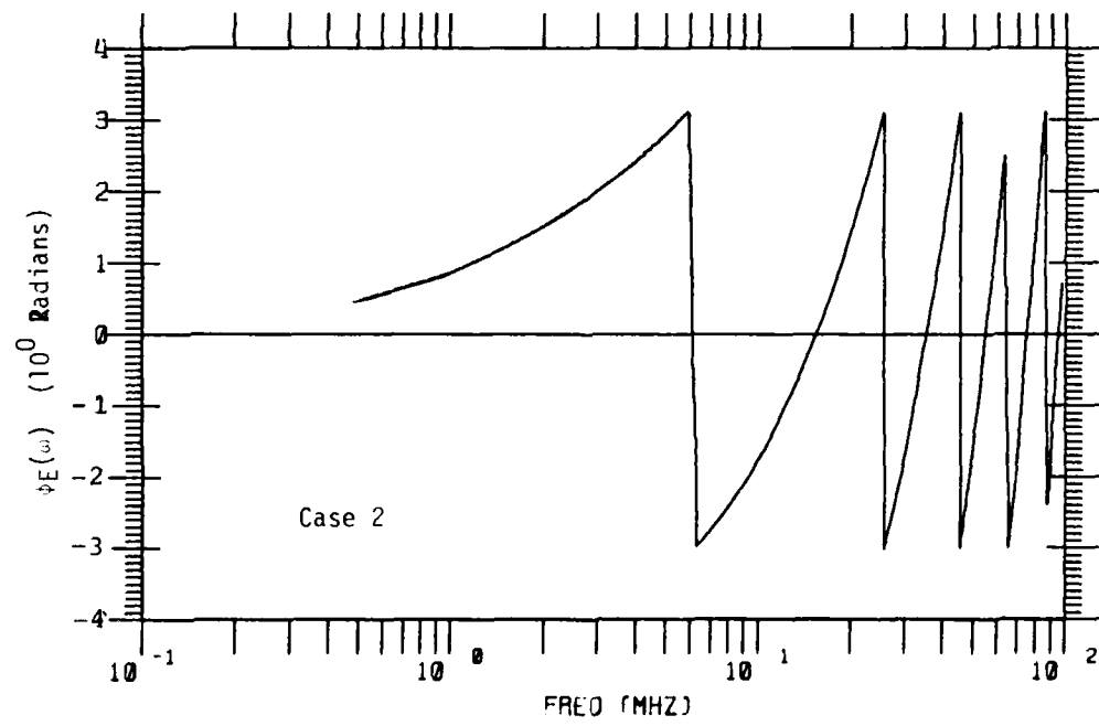
Figure 11b. Phase for the Incident Electric Fields
