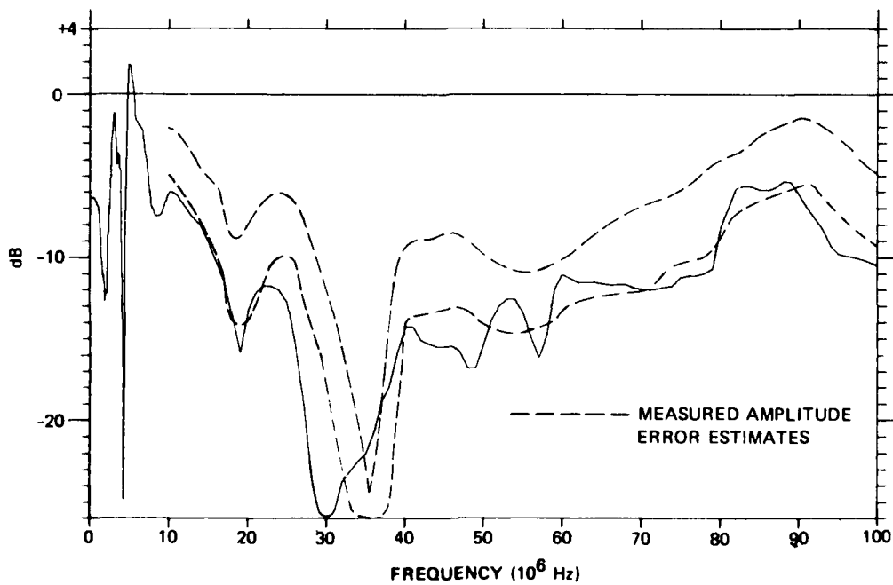
Figure 33b. 45° Polarization Calculated Amplitude (100 MHz)
