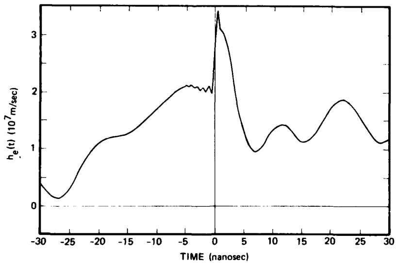
Figure 1b. h_e(t) for the Horizontally Polarized Data
