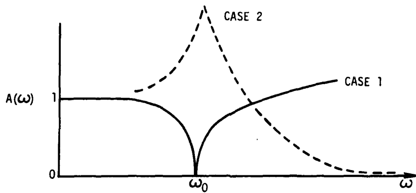
Figure 22b. Amplitude for \pi Shift in Phase
