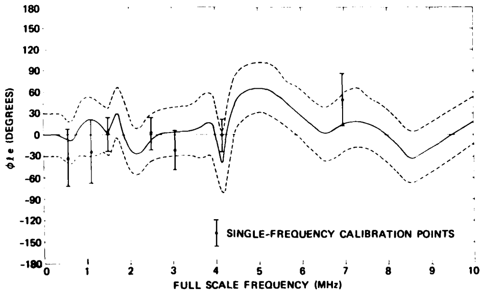
Figure 28b. Effective Length 45 Degree Polarization (Final)
