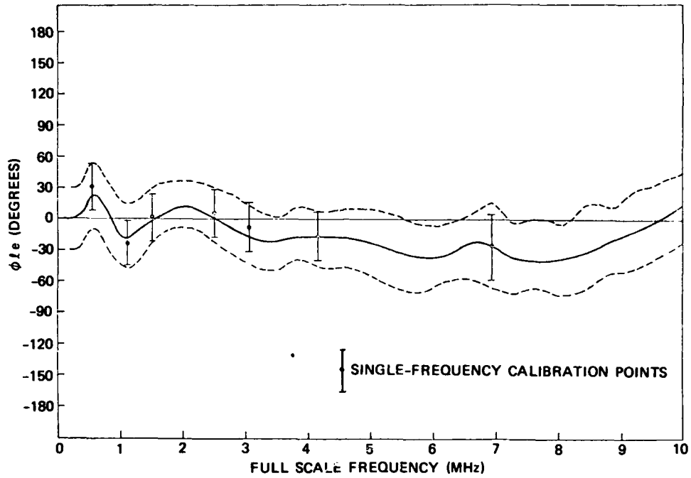
Figure 27a. Effective Length Phase Vertical Polarization (Preliminary)
