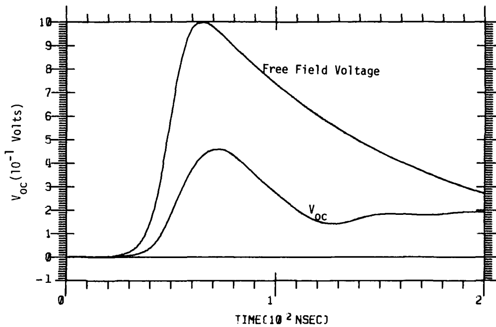
Figure 14a. Open Circuit Voltage for Vertical Case 2 Electric Field (200 nsec)
