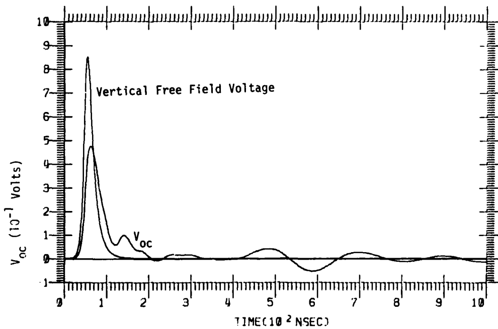
Figure 17b. Open Circuit Voltage for 30° Polarized Case 1 Electric Field (1 \mu sec)
