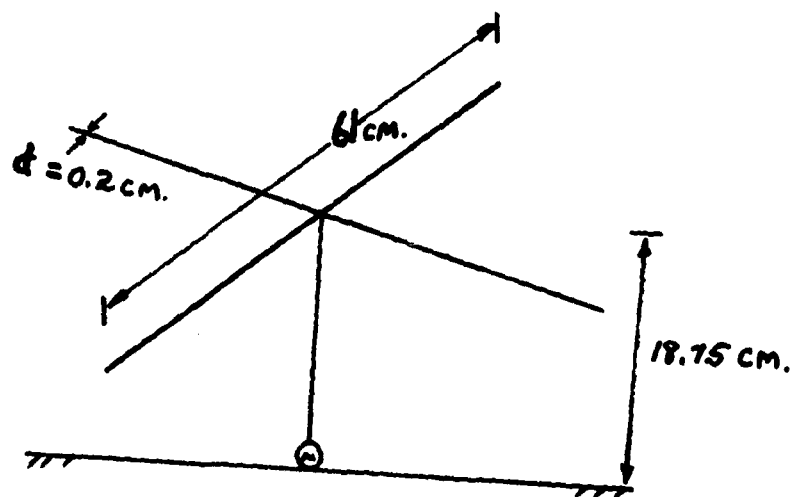
Fig. 15a Model of Top-Loaded Monopole for Numerical Analysis
