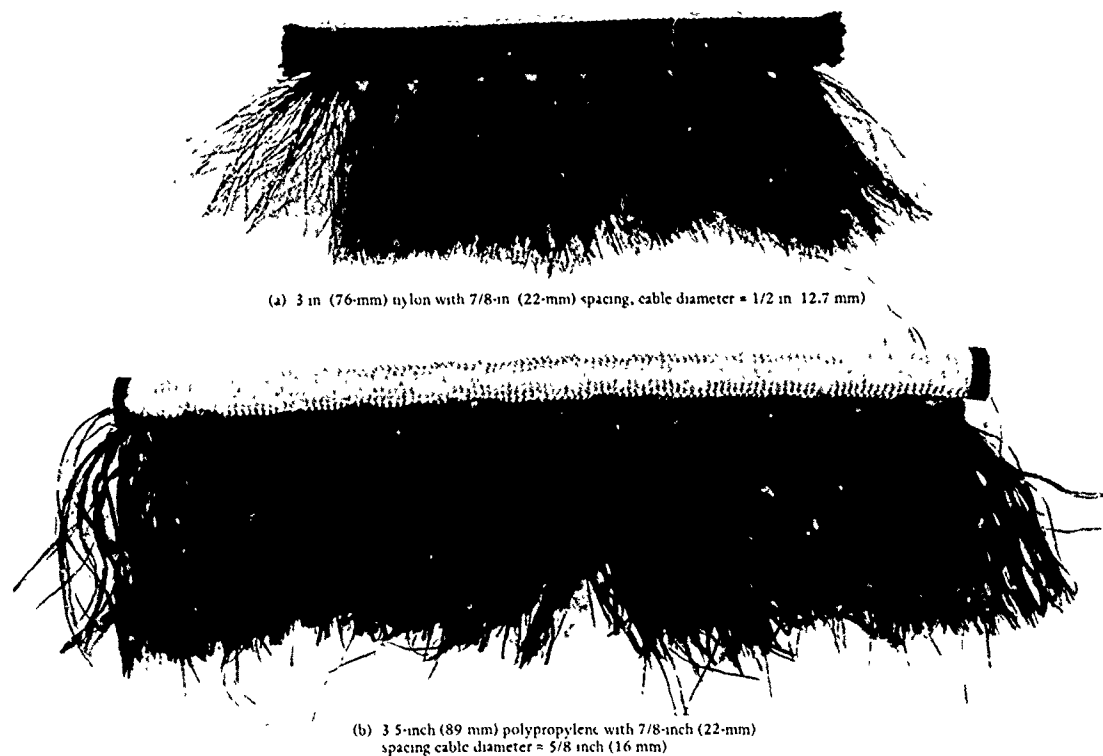
Figure 1. Wall Rope Works fringe fairing.
